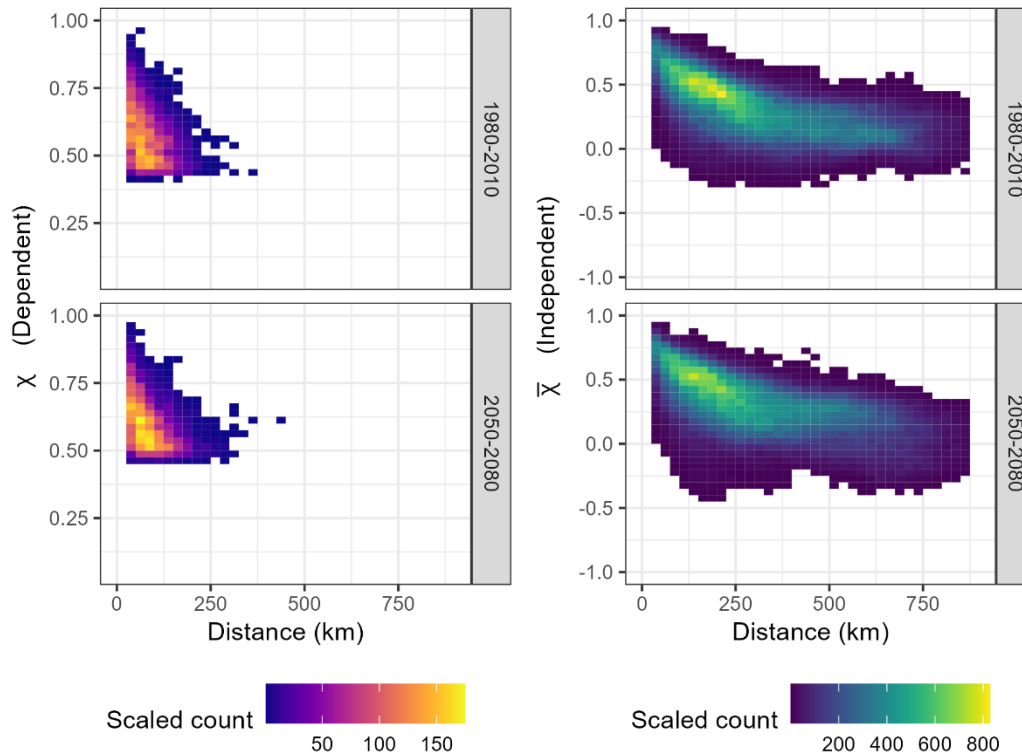
Figure 87 Heatmaps showing asymptotic dependence for 100 000 random pairs of points on the river network. \chi is only shown for pairs of locations which are asymptotically dependent based on \bar{\chi} > 0.99 .
