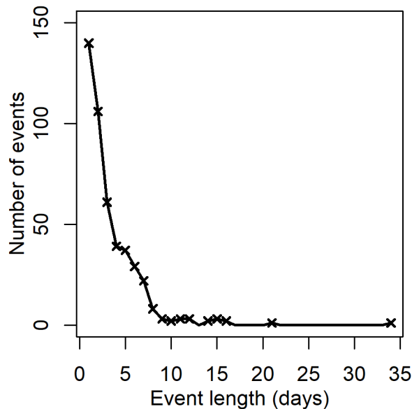
160 Figure 24 Number of events with different durations, based on 0.5% coverage and at-site exceedance of two days per year.
