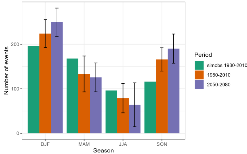
Figure 54 Number of widespread events, summed across ensemble members, split by season and time-slice. Left: total events, Right: mean number of events per ensemble member with error bars showing minimum and maximum across ensemble members.
