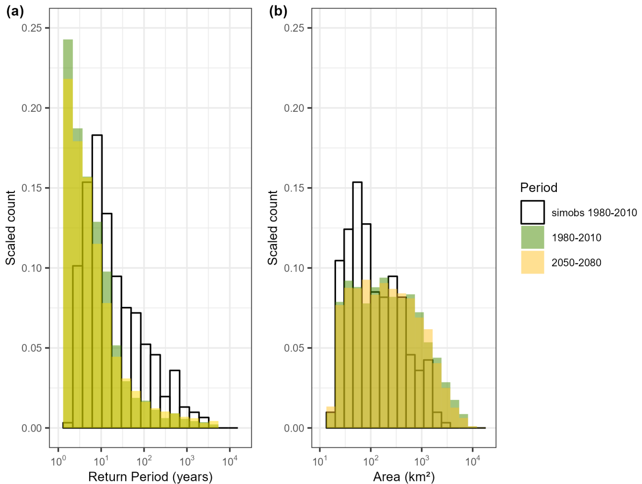
240 Figure 43 Histograms showing distribution of event area and return period, split across time-slices and ensemble members.
