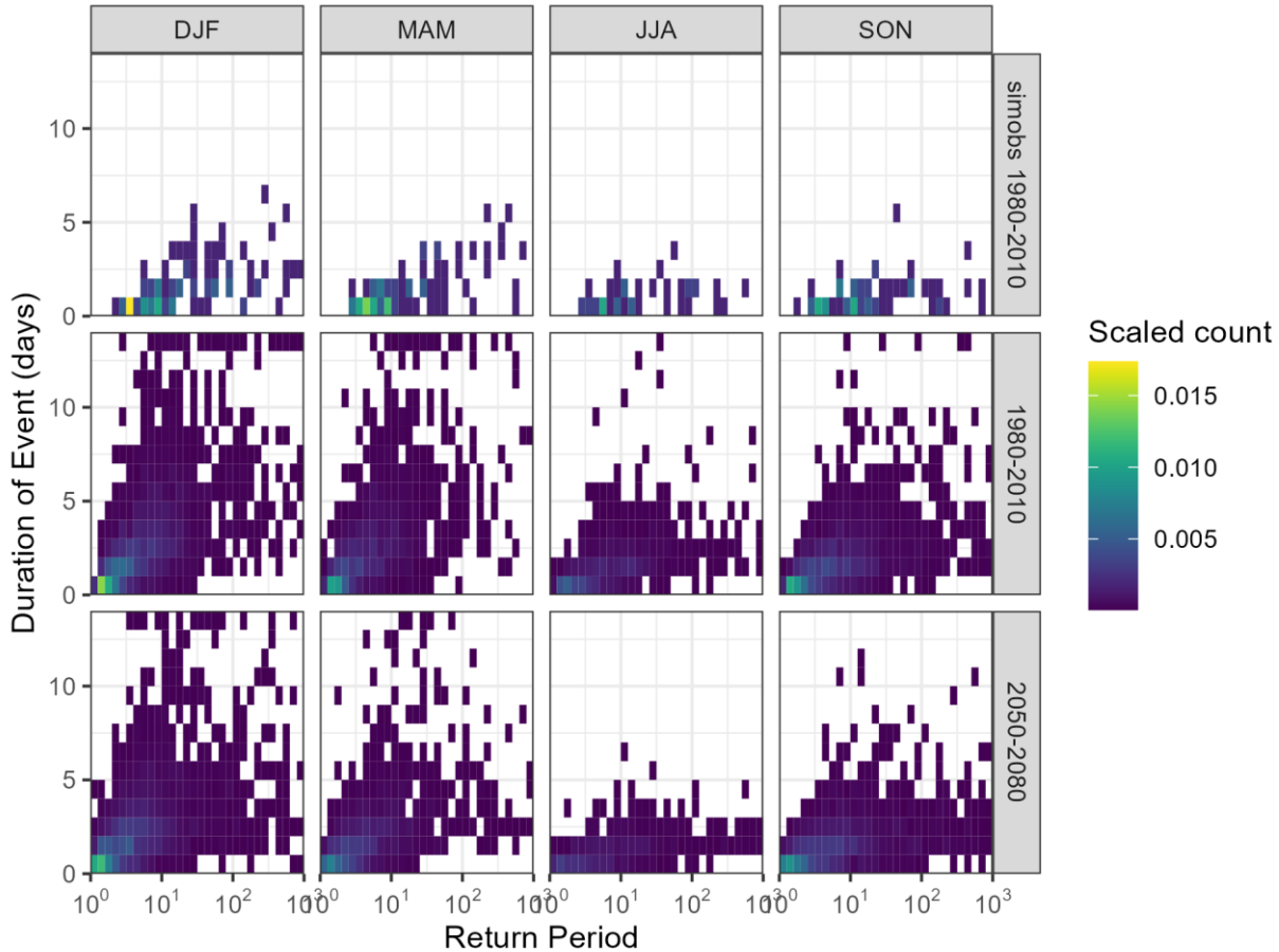
Figure 65 Heatmaps showing joint distribution of return period and event duration, summed across ensemble members, split by season and time-slice. Count is scaled so that the total of events in each timeslice adds up to 1.
