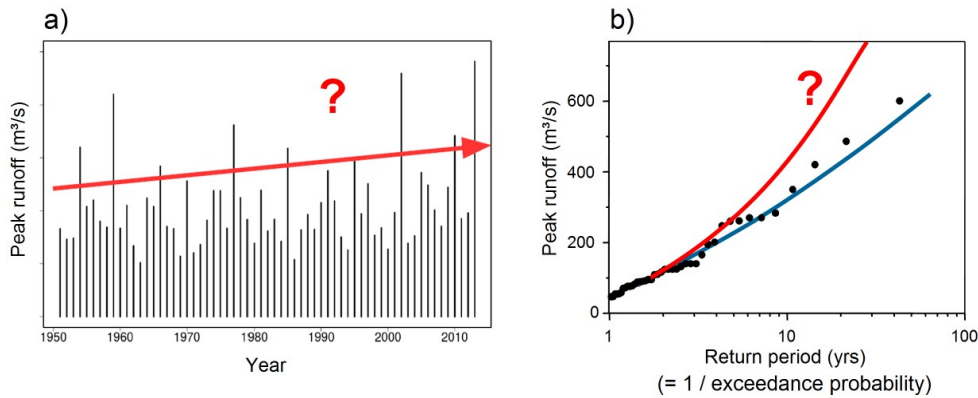
105 Figure 1. (a) A hypothetical river flood time series. Each bar is the maximum annual peak runoff, and the red arrow indicates an increase in hazard. (b) Flood frequency plot. Each point is the maximum annual peak runoff plotted against its exceedance probability (expressed as its inverse, the return period). Blue fitted line reflects the past situation, the red line a potential increase in river flood hazard. ‘Hazard’ is defined as the exceedance probability of a river flood level that potentially causes damage.
