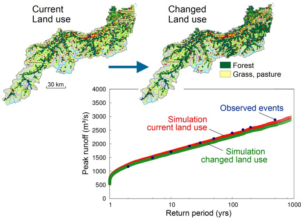
Figure 6. Effects of afforestation on floods for the 9700 km 2 Inn catchment at Oberaudorf in Austria using a distributed rainfall runoff model. Given the catchment area is large, the relevant runoff generation mechanism is saturation excess and thus the effect of land use change (an additional 100 000 ha of forest) is small. The flood peak runoff associated with a return period of 100 yrs is reduced by only 4%. Blöschl et al. (2018).
