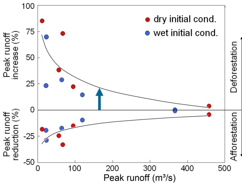
205 Figure 4. Effect of land use change on flood peak runoff for the 622 km 2 Kamp catchment at Zwettl in Austria, using a distributed rainfall-runoff model. Upper part of the figure: increase in peak runoff of a scenario of complete deforestation relative to the observed baseline case of 47% forested area, plotted against the peak runoff of the baseline case. Lower part of the figure: same but for afforestation (increase in forested area from 47% to 86%). Each point represents one event, and the initial soil moisture is shown as colour. Deforestation reduces infiltration and thus increases surface runoff. The effect decreases as the event magnitude increases. Modified from Salazar et al. (2012).
