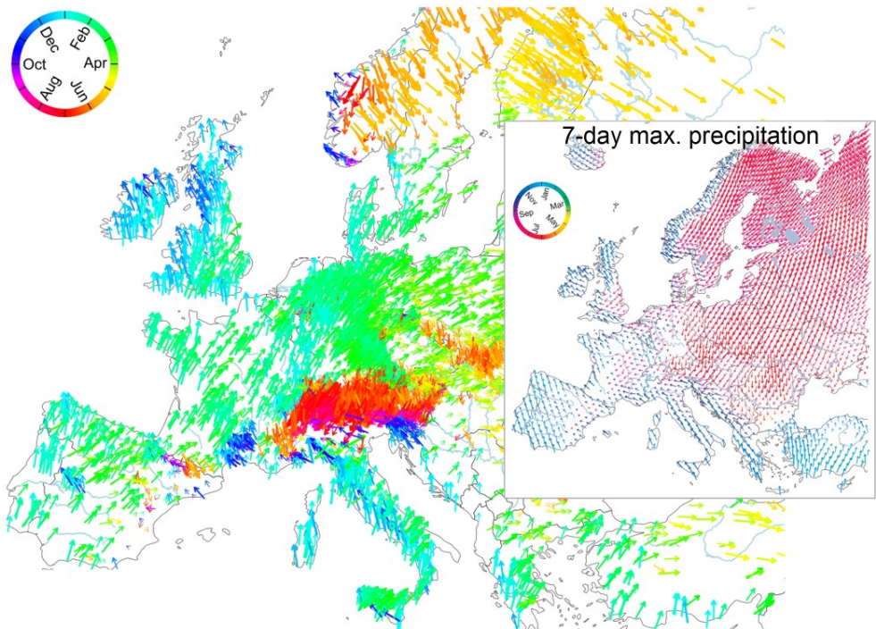
Figure 15. Average timing of floods within the year to understand changes in flood hazard. Blue arrows pointing upwards indicate winter floods, red arrows downward summer floods. Based on data from 4062 stations, 1960-2010. Inset image shows a similar plot, but for 7-day maximum annual precipitation based on the eobs data set. The flood seasonality differs significantly from that of precipitation, which is because of the seasonal interplay of soil moisture, snow and extreme precipitation. Blöschl et al. (2017).
