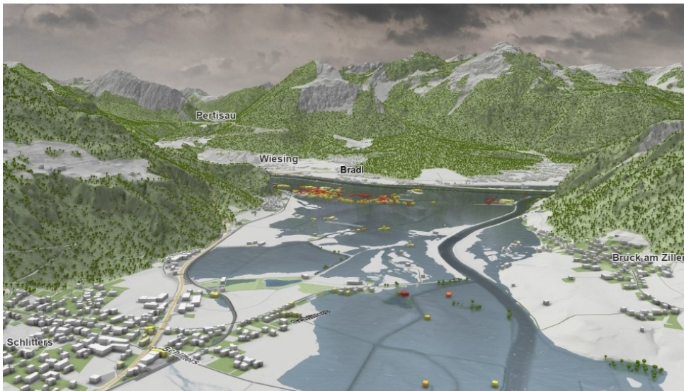
290 Figure 7. Flood inundation modelling at hyper-resolution in Austria using a two dimensional hydrodynamic model at 2 m resolution nationwide. The flood hazard zones are associated with a return period of 100 years of the peak runoff. Published by the Ministry of Agriculture, Regions and Tourism as part of the HORA flood risk zoning project on https://www.hora.gv.at (website visited on 1 June, 2022). Blöschl et al. (2022).
