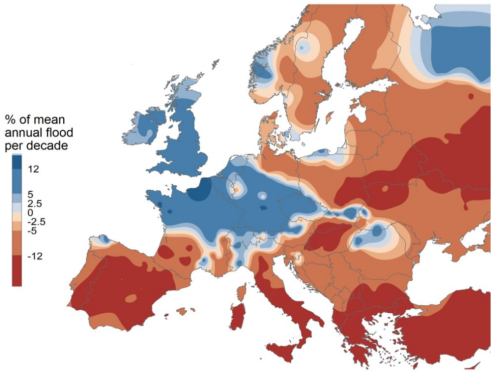
450 Figure 13. Observed flood trends in the period 1960-2010 based on the analysis of runoff data. Blue colours indicate an increasing trend and reddish colours a decreasing trend in the median flood peak runoff. Only stations with significant trends (significance level \alpha = 0.1 ) were used in the spatial interpolation (664 stations). Blöschl et al. (2019).
