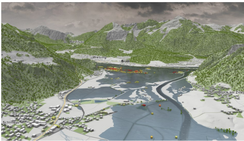
Figure 7. Flood inundation modelling at hyper-resolution in Austria using a two dimensional hydrodynamic model at 2 m resolution nationwide. The flood hazard zones are associated with a return period of 100 years of the peak runoff. Published by the Ministry of Agriculture, Regions and Tourism as part of the HORA flood risk zoning project on https://www.hora.gv.at (website visited on 1 June, 2022). Blöschl et al. (2022).
