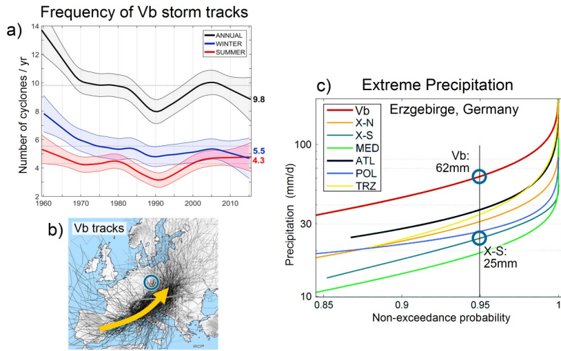
Figure 14. (a) Frequency of Vb storm tracks in the period 1960-2020. (b) Vb tracks (according to Van Bebbler, 1891) follow a path across the western Mediterranean into central Europe and are responsible for some of the largest floods on record, such as the August 2002 and June 2013 floods. (c) Vb storms produce much larger heavy precipitation than other track types, as illustrated by the frequency distribution of daily precipitation in the Erzgebirge region, Germany. X-S are storm types that approach from the southeast. Cyclone track analysis based on a combination of sea level and 700hPa pressure from JRA-55 reanalysis data. Hofstätter et al. (2016, 2018); Hofstätter and Blöschl (2019).
