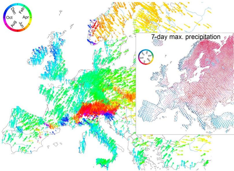
Figure 15. Average timing of floods within the year to understand changes in flood hazard. Blue arrows pointing upwards indicate winter floods, red arrows downward summer floods. Based on data from 4062 stations, 1960-2010. Inset image shows a similar plot, but for 7-day maximum annual precipitation based on the eobs data set. The flood seasonality differs significantly from that of precipitation, which is because of the seasonal interplay of soil moisture, snow and extreme precipitation. Blöschl et al. (2017).
