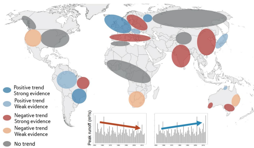
435 Figure 11. Observed flood trends in the period of approximately 1960-2010 based on the analysis of runoff data. Blue colours indicate an increasing trend, reddish colours a decreasing trend in mean flood peak runoff. The patterns are based on a literature meta-analysis. Globally, there are both increasing and decreasing trends of flood hazard. Merz et al. (2021).
