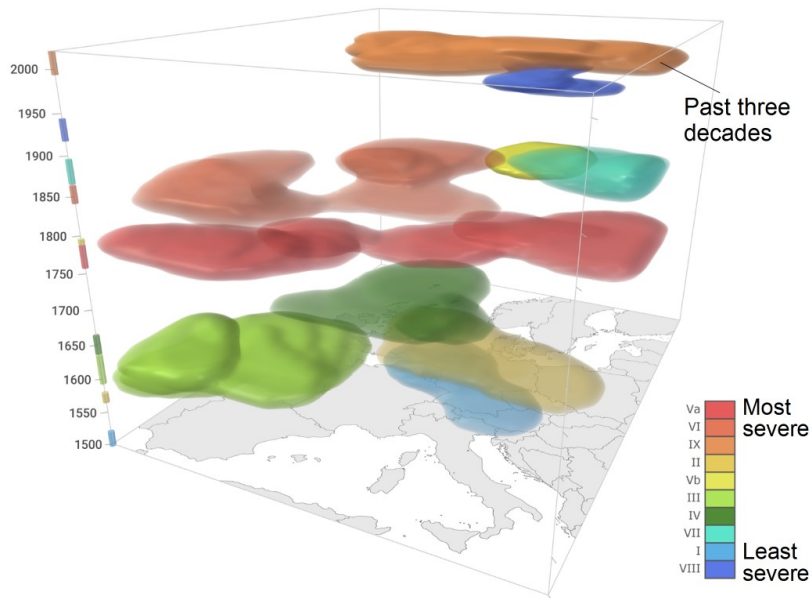
Figure 12. Flood-rich periods in last 500 years in Europe defined as periods and regions in which floods are much larger and more frequent than usual. The flood-rich periods were identified from 103 high-resolution historical flood series based on documentary evidence. The past three decades were among the most flood-rich periods. Blöschl et al. (2020).
