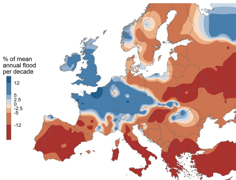
Figure 13. Observed flood trends in the period 1960-2010 based on the analysis of runoff data. Blue colours indicate an increasing trend and reddish colours a decreasing trend in the median flood peak runoff. Only stations with significant trends (significance level \alpha = 0.1 ) were used in the spatial interpolation (664 stations). Blöschl et al. (2019).
