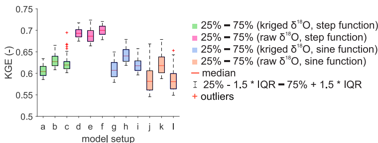
Figure 5. Boxplot of model performance ranges in behavioral solutions. The letters on the x-axis refer to the model setup type according to Table 1. Boxplots filled with the same colors represent model setups characterized by the same interpolation scheme in space and time. On each box, the central red line indicates the median, and the bottom and top edges of the box indicate the 25th and 75th percentiles respectively, namely the interquartile range (IQR). The whiskers extend to the most extreme data points not considered outliers which are 25th percentile minus 1.5 times IQR and 25th percentile plus 1.5 times IQR, respectively. The outliers are plotted individually using the red '+' mark.
