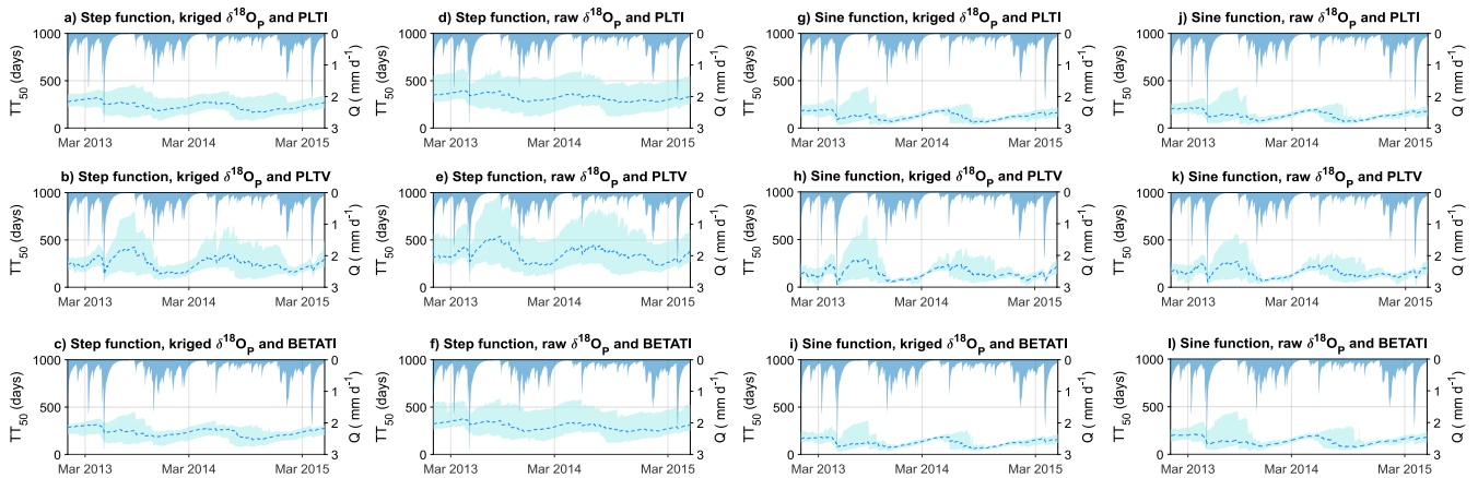
Figure 6. Predicted TT_{50} of streamflow; the light blue line and the shaded area represent, respectively, the ensemble mean of all possible solutions and their range according to the 95% CI.
