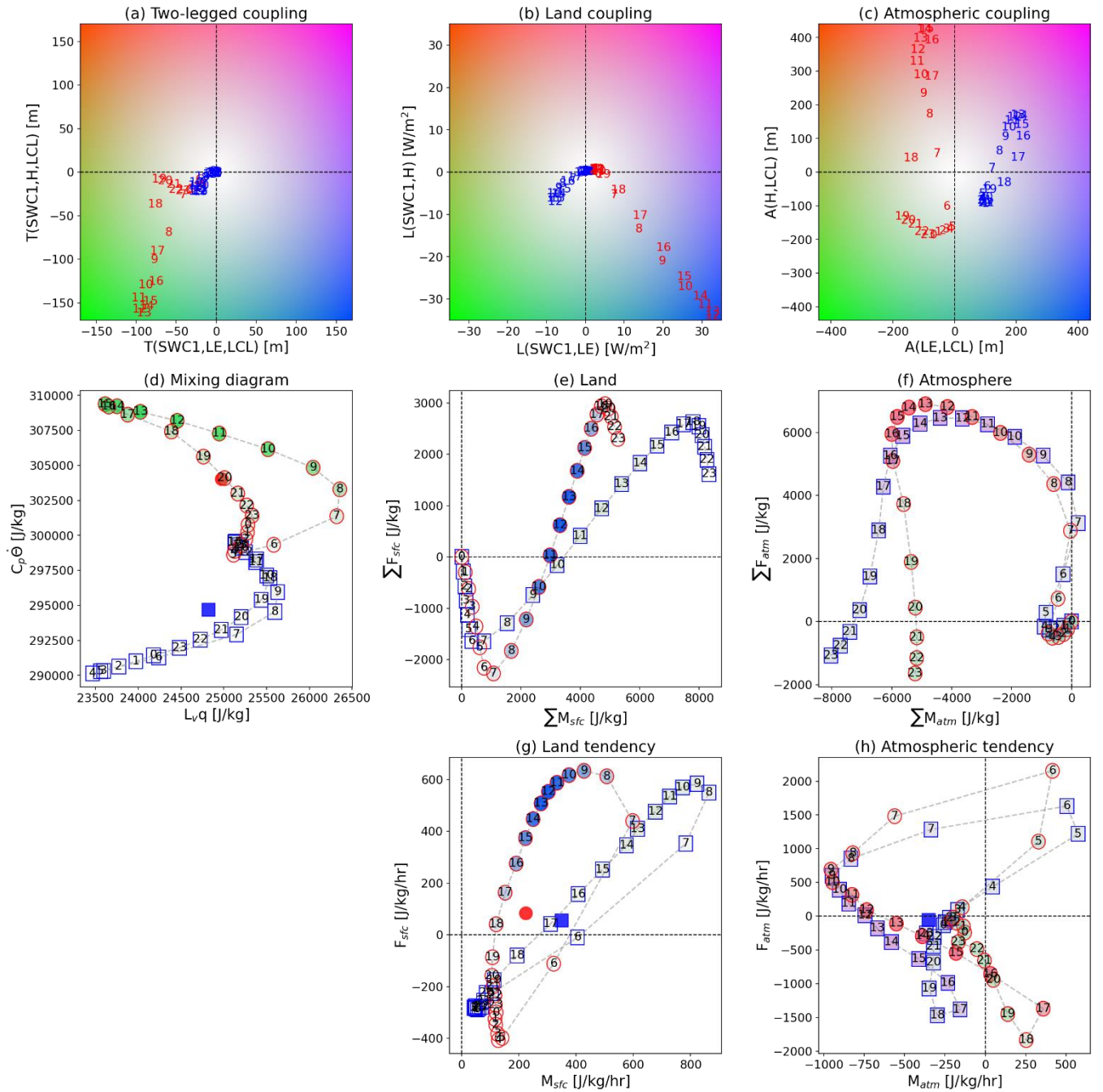
Figure 5: Same as Fig. 4, but for the sensitivity of water-limited (circles outlined in red) and energy-limited (squares outlined in blue) regimes sampled by upper and lower 10% sites (N=23) as described in section 3.3.
