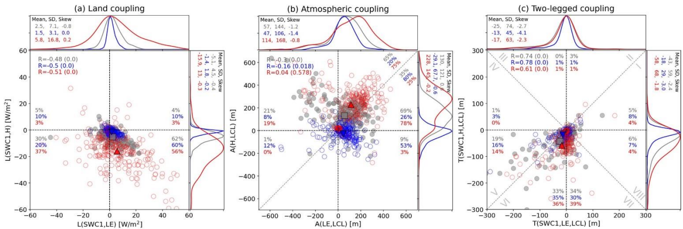
Figure 2: Scatter plot of (a) land coupling, (b) atmospheric coupling, and (c) two-legged coupling for daily (grey), midday averaged (11–13 LST; red) and midnight averaged (23–01 LST; blue) values at 230 flux sites. Squares, upward triangles, and downward triangles indicate the mean across 230 sites for daily, midday, and midnight, respectively. Correlations and corresponding p-values (bracketed) are denoted in the upper-left corners. On each scatter diagram, percentages of stations in each quadrant (each octant for panel c) are indicated for daily, midday, and midnight data with corresponding colours. For the atmospheric coupling, percentages are also indicated on either side of the diagonal ( y=x ) line. The distribution of the kernel density estimations corresponding to x- and y-axis is shown as marginal distributions along the upper and right sides of each scatter plot. Each is normalized to have the same maximum value; the mean, standard deviation, and skewness for each distribution are also shown.
