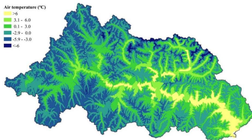
680 Figure A2: Mean annual temperature (°C).
