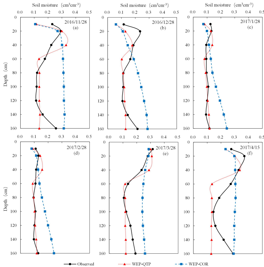
425 Figure 9: Simulated (WEP-QTP and WEP-COR models) and observed moisture contents of the soil-gravel layer during the freezing and thawing periods.
