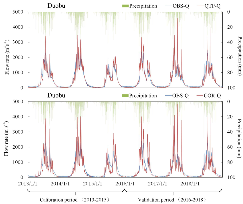
380 Figure 6: Verification results of the WEP-QTP and WEP-COR models at (a) Duobu, (b) Gongbujiangda, and (c) Baheqiao stations.
