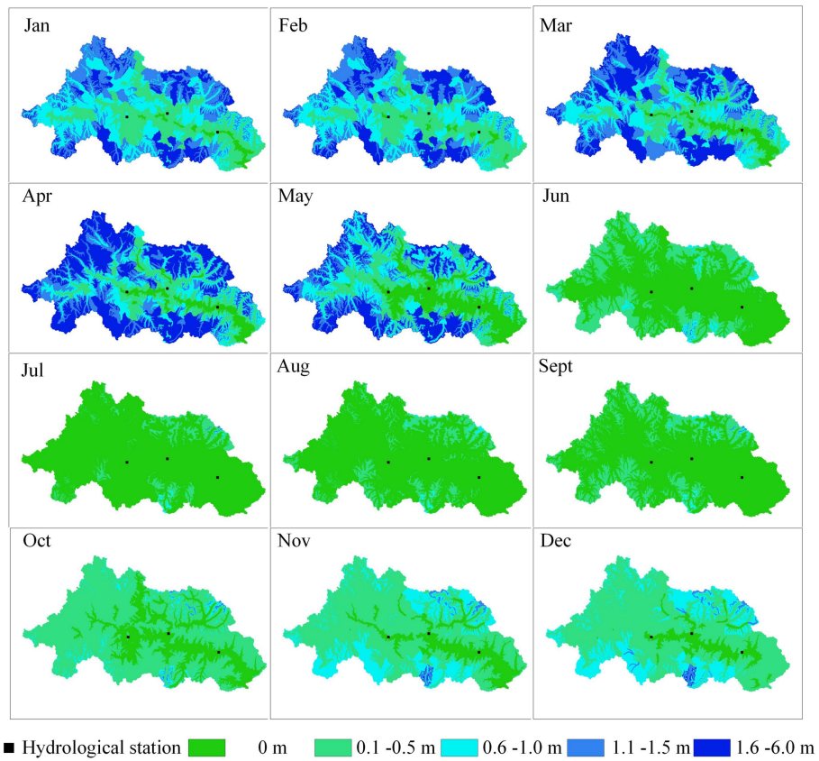
Figure 12: Spatiotemporal variation in snow cover thickness in 2014.
