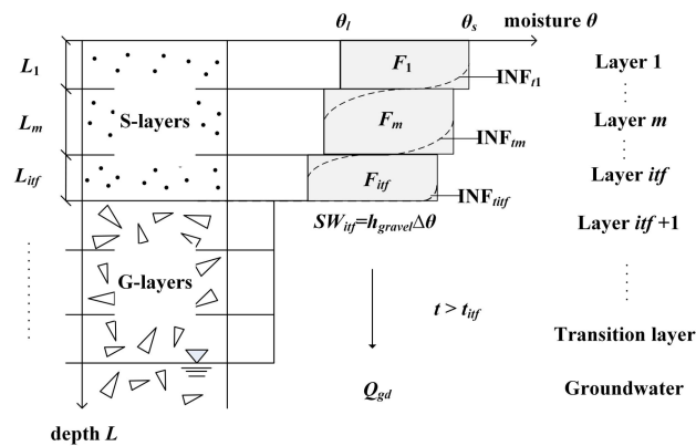
250 Figure 5: Cumulative infiltration process of the WEP–QTP model.
