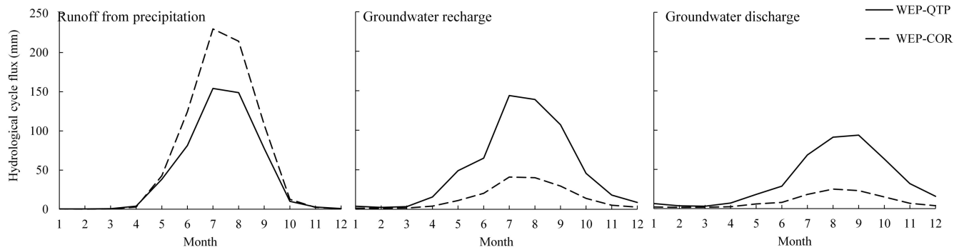
475 Figure 11: Monthly changes in hydrological cycle flux simulated by the WEP-QTP and WEP-COR models.
