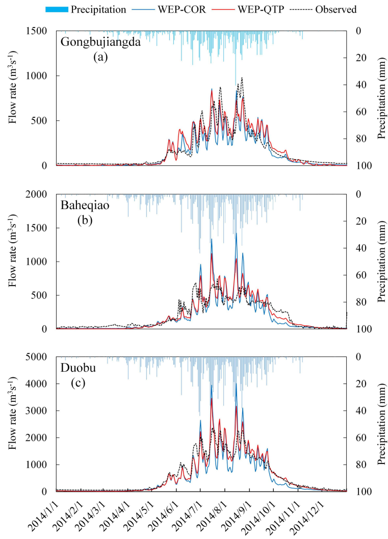
Figure 10: Simulated (WEP-QTP and WEP-COR models) and observed flow rates at (a) Gongbujiangda, (b) Baheqiao, and (c) Duobu stations in 2014.
