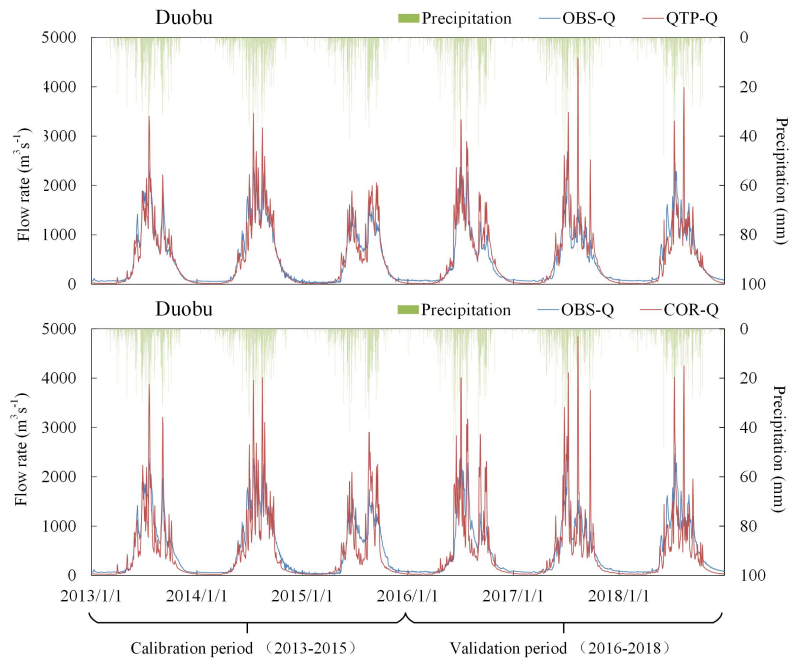
Figure 6: Verification results of the WEP-QTP and WEP-COR models at (a) Duobu, (b) Gongbujiangda, and (c) Baheqiao stations.
