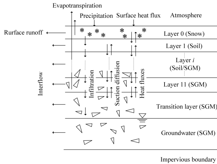
Figure 3: Layered calculation structure of the dualistic "soil-gravel" structure (a), snow-soil-gravel layered structure (b) and the "snow-soil-gravel layer" continuum (c)
