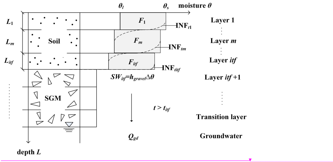
Figure 4: Cumulative infiltration process of the WEP-QTP model
