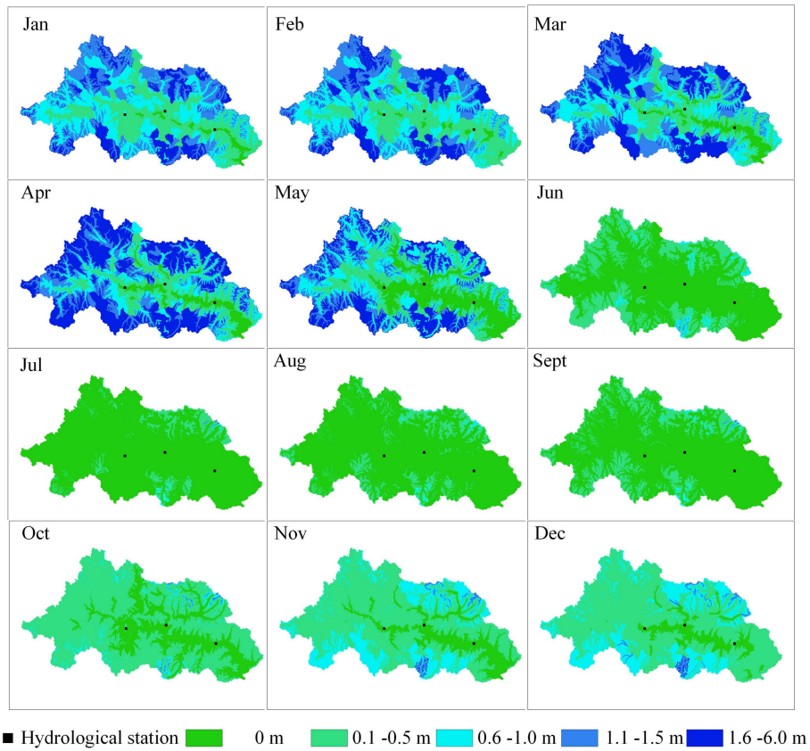
475 Figure 11. Temporal and spatial variation of snow cover thickness in 2014
