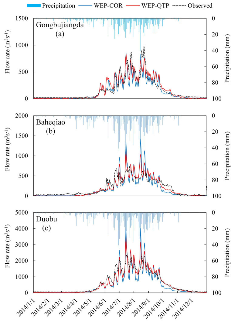
445 Figure 9: Simulated (WEP-QTP and WEP-COR models) and observed flow rates at (a) Gongbujiangda, (b) Baheqiao, and (c) Duobu stations in 2014
