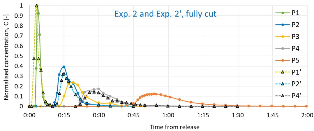
Figure A1. Tracer concentrations in measured cross-sections normalised with the maximum concentration in the first cross-section P1. Fully cut conditions, original Exp. 2 (cross-sections P1, P2, P3, P4 and P5) and repeated experiment Exp. 2’ (cross-sections P1’, P2’ and P4’).
