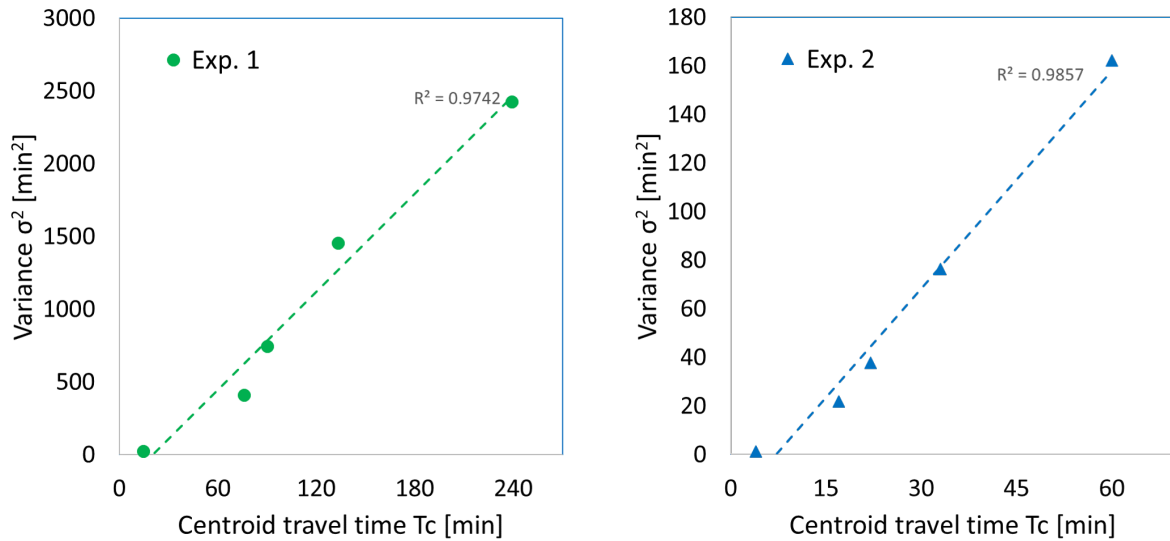
Figure 9. Variance ( \sigma^2 ) of the temporal concentration distributions against the centroid travel time ( T_c ) for Exp. 1 (left) and Exp. 2 (right).
