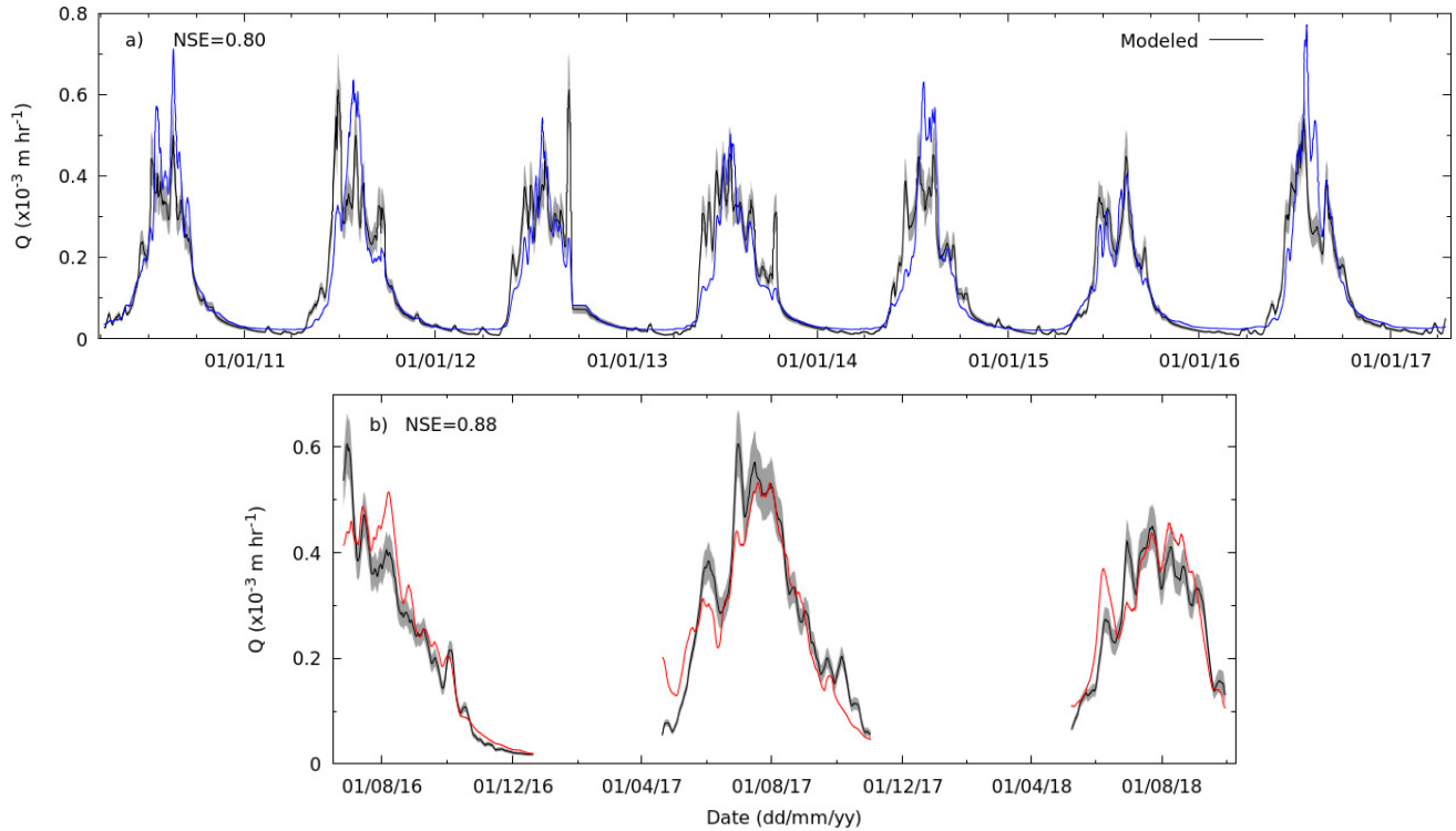
Figure 5. Modelled weekly runoff (black lines, with grey bands denoting 2- \sigma uncertainty) compared with the corresponding observations for (a) upper Dudhkoshi (blue solid line), and (b) Chandra (red solid line) catchments.
