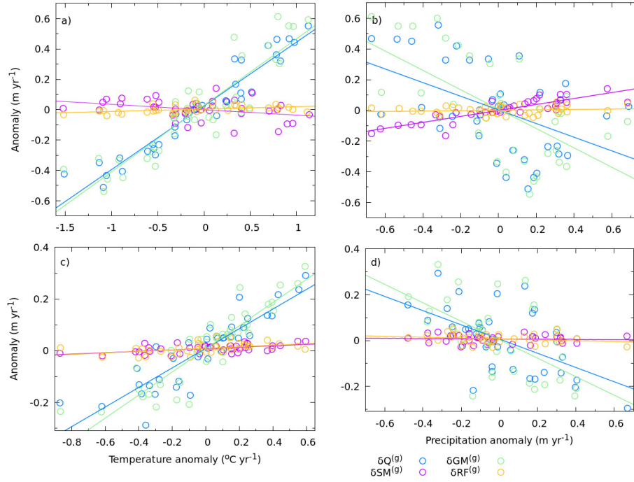
Figure 7. The anomalies of glacier runoff \delta Q^{(g)} , and its components, namely, snowmelt \delta SM^{(g)} , glacier ice melt \delta GM^{(g)} , and rainfall \delta RF^{(g)} for the glacierised parts of the catchments are plotted as a function of the corresponding temperature and precipitation anomalies: (a, b) for Chandra catchment, and (c, d) for upper Dudhkoshi catchment. The corresponding best-fit straight lines are also shown.
