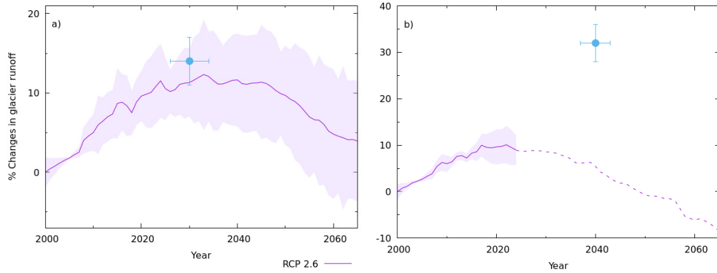
Figure 9. The ‘peak water’ due to future glacier changes predicted using Eq.(15) for (a) Chandra, and (b) upper Dudhkoshi catchments, respectively. The solid sky-blue dots represents the corresponding ‘peak water’ as reported in Huss and Hock (2018) for both the catchments. Dashed portion of the solid line in upper Dudhkoshi catchment indicate the corresponding temperature change beyond the calibration range of the catchment. See text for details.
