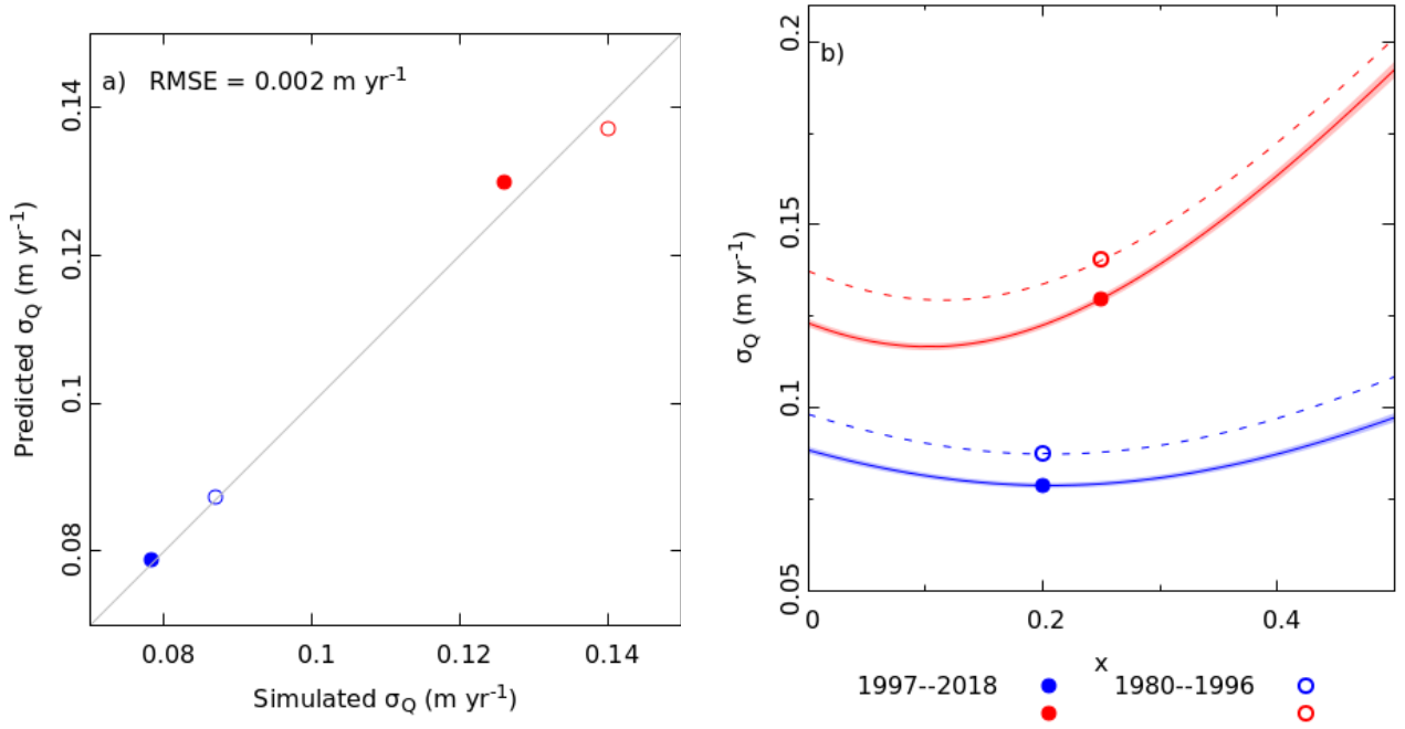
Figure 8. a) Predicted \sigma_Q using Eq.(14) are compared with the corresponding simulated values for both the catchments. The solid and open circles denote data for the periods 1997–2018 and 1980–1996, respectively. Data for Chandra and upper Dudhkoshi catchments are shown with red and blue symbols, respectively. b) The solid (dashed) lines show \sigma_Q(x) obtained using \sigma_T and \sigma_T values from 1997–2018 (1980–1996).
