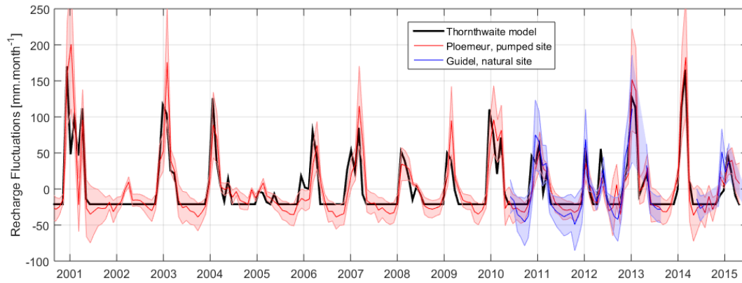
Figure 8. Monthly recharge fluctuations estimated from groundwater analytical model at different boreholes on the Ploemeur (in red) and Guidel (blue) sites, propagating model parameter uncertainties. Shaded areas represent GW model uncertainty and variability between the different observation wells. Black line represents potential recharge fluctuations (anomalies compared to the mean value) from the Thornthwaite model.
