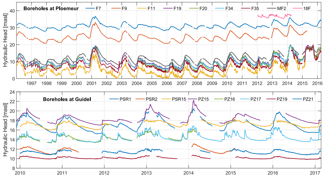
Figure 3. Observed GW level variations in boreholes at Ploemeur pumping site (upper graph) and Guidel 'natural' site (lower graph) observatories . Note the difference in scales between the two sites. masl refers to meters above sea level.
