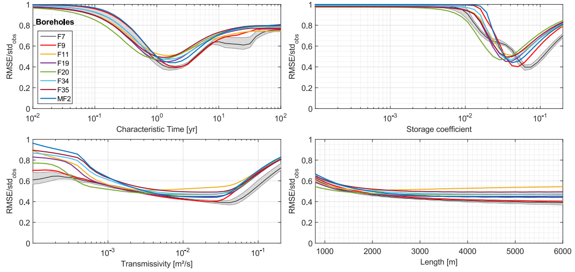
Figure 6. Evolution of the minimal normalized RMSE for Ploemur wells as a function of model parameters: characteristic time, storage coefficient (top-right), transmissivity (bottom-left) and aquifer length (bottom-right). Evolution of characteristic time, a combination of the three parameters, is plotted on the top-left graph. We selected the best prescribed potential recharge model for each point. The impact of the prescribed recharge is drawn by the shaded area on borehole F7.
