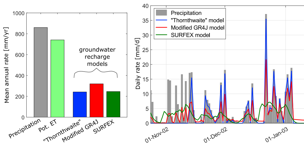
Figure 4. On the left: mean annual precipitation, potential evapotranspiration rate, and estimated potential recharge rates from Thornthwaite, GR4J and SURFEX models on Ploemeur-Guidel sites (1996-2017). On the right: estimated daily potential recharge rates from Thornthwaite, GR4J and SURFEX models from November 2002 to January 2003. Daily precipitation (grey shaded bars) is recorded by a METEO-FRANCE weather station and is used to derive recharge from Thornthwaite and GR4J models.
