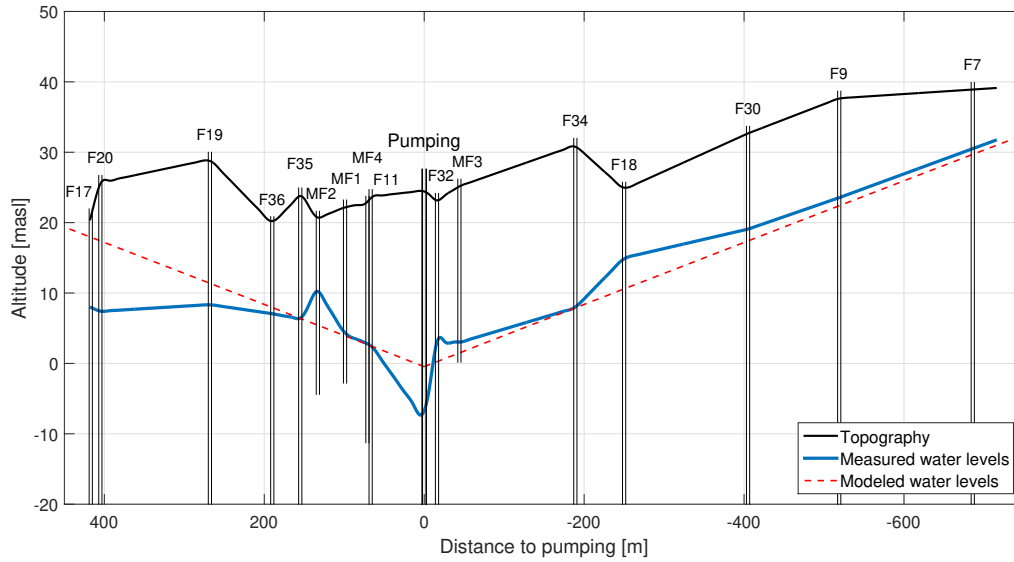
Figure C1. Mean groundwater levels observed on the Ploemur pumping site (blue curve), shown on a SE-NW cross section. The red dashed curve represents the best 1D steady-state analytical model which has the lowest least square difference between data and model.
