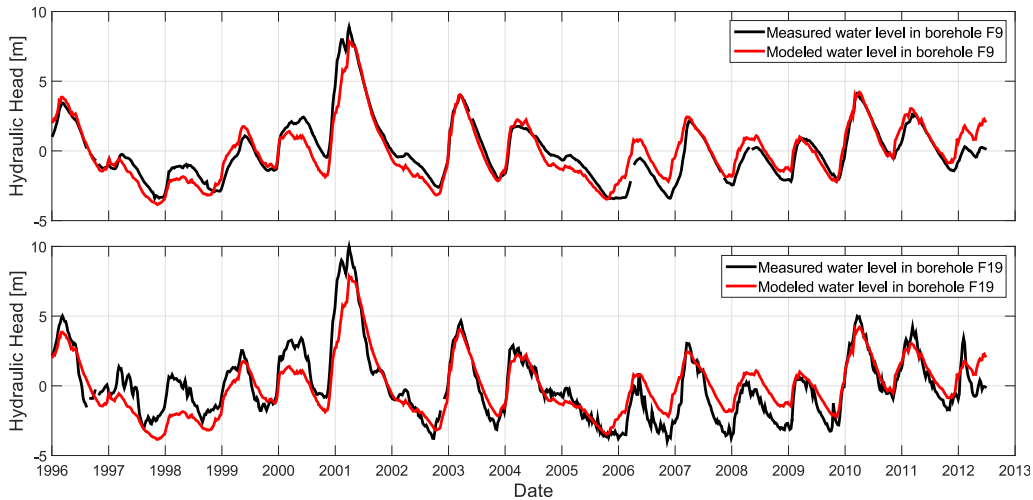
Figure 5. Comparison between best modeled and observed water table fluctuations at borehole F9 (upper graph) and F19 (lower graph), respectively at 519 m and 268 m of Ploemeur’s pumping wells. Hydraulic parameters correspond to best parameters (lowest RMSE on Figure 6 regarding water table fluctuations). Prescribed recharge fluctuations have negligible impact on these parameters and the quality of the fit.
