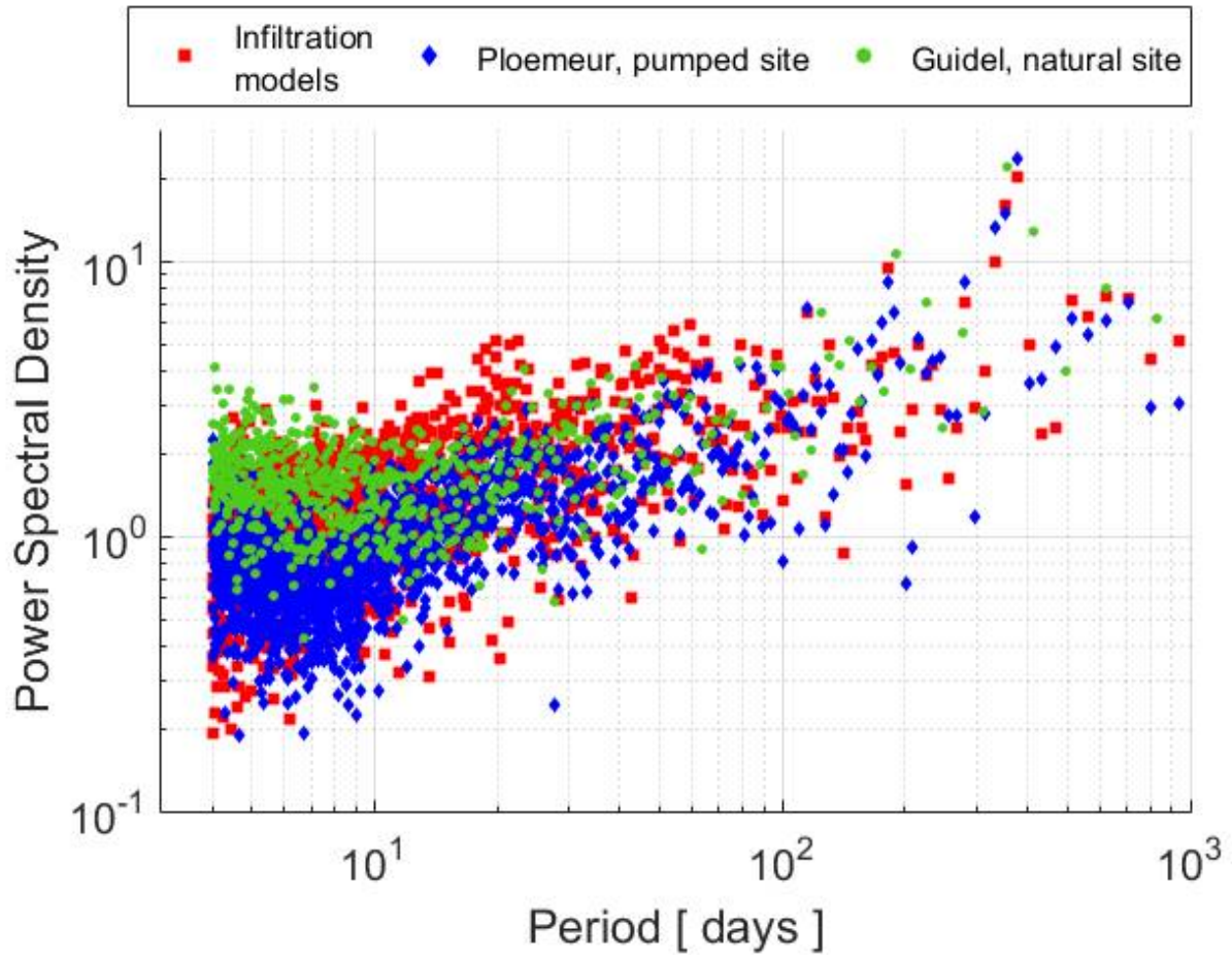
Figure 1: Power spectrum of recharge estimated from infiltration models and from groundwater levels fluctuations in Ploemeur and Guidel sites.
