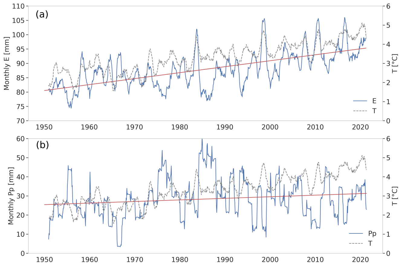
Figure 10. 12-month moving average monthly total evaporation (a) and precipitation (b), and 2-m mean air temperature over the saline lake of Salar del Huasco from 1950 to 2020. The long-term trend is indicated by the red line.
