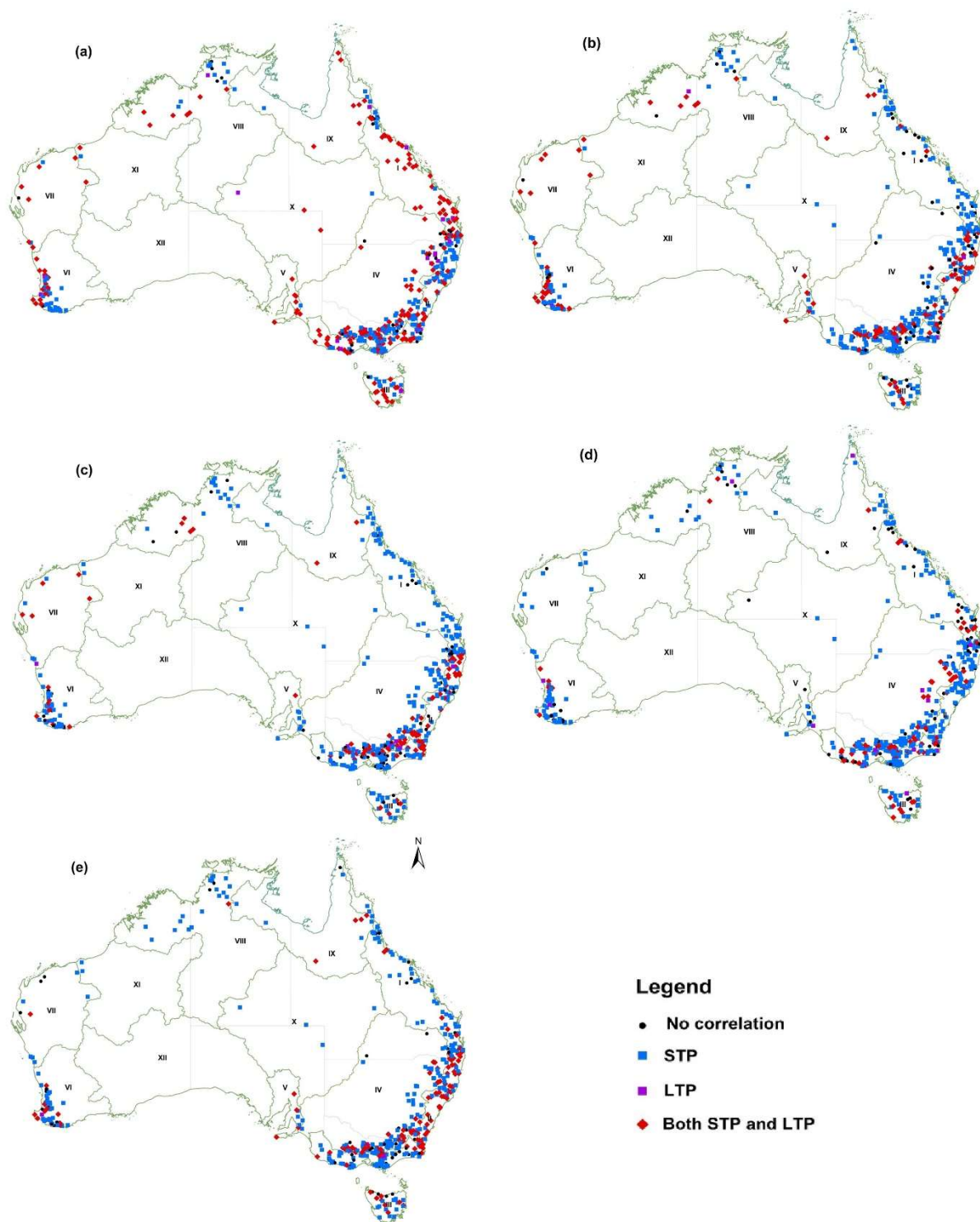
460 Figure 6: Spatial distribution of stations where streamflow shows persistence, Short Term (STP) and Long Term (LTP), in (a) autumn (Mar-May), (b) winter (Jun-Aug), (c) spring (Sep-Nov), (d) summer (Dec-Feb), and (e) annual (water year) at p < 0.10 .
