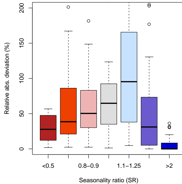
Figure 7. Performance gain by seasonality ratio classes of Laaha and Blöschl (2006b). Shown are the relative absolute deviations ( rad_T ) for the T=100 year event. The colour coding is that of Fig. 6.
