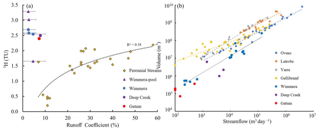
Figure 9. (a) Comparison of ^3\text{H} activities and runoff coefficients at low and zero flow conditions and (b) volumes of water sustaining streamflows between the upper Wimmera River and other intermittent and perennial streams in southeast Australia. Error bars represent the uncertainty of annual rainfall in the upper Wimmera Catchment. Perennial streams are the Ovens, Latrobe, Yarra, and Gellibrand (data from Cartwright et al., 2020); intermittent streams are Deep Creek and Gatum (data from Cartwright and Morgenstern, 2016 and Barua et al., 2022).
