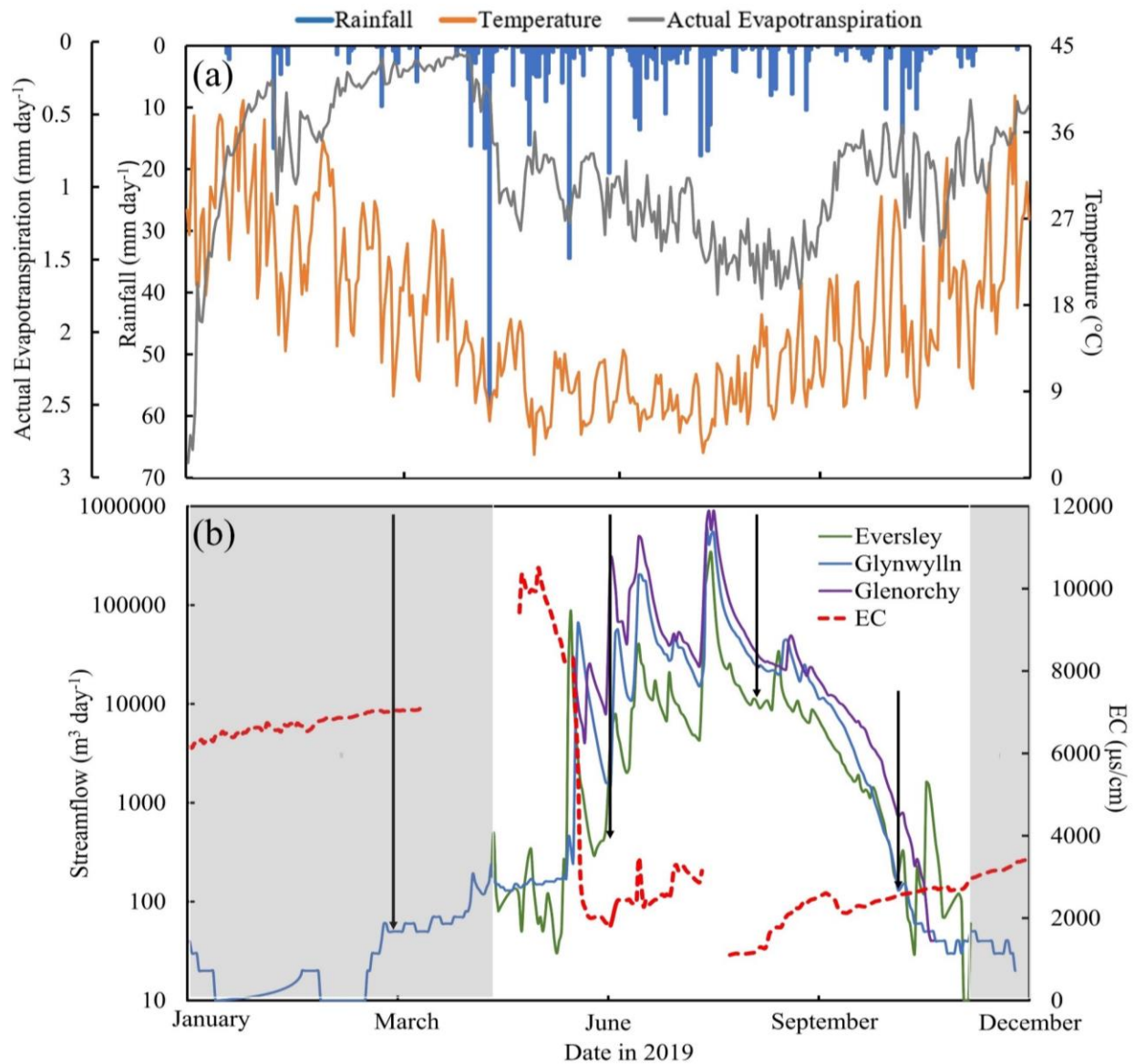
325 Figure 2. (a) Variations in daily rainfall, daily actual evapotranspiration, and temperature and (b) EC at 330 Glynwylln (missing data are caused by measurement errors of equipment) and streamflow at Eversley, Glynwylln, and Glenorchy (Fig.1) in the upper Wimmera River in 2019. Variations in EC at Glynwylln (missing data are caused by measurement errors of equipment) and streamflow at Eversley, Glynwylln, and Glenorchy (Fig.1) in the upper Wimmera River in 2019. Sampling times are indicated by arrowed lines. Shaded areas represent the zero-flow periods. Data from Department of Environment, Land, Water and Planning (2021) and Bureau of Meteorology (2021).
