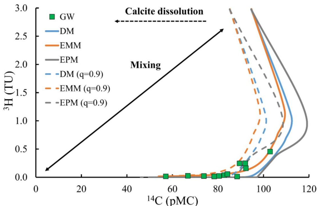
390 Figure 5. ^3\text{H} activities vs. ^{14}\text{C} activities of groundwater from the upper Wimmera River. Curved lines are the predicted covariance in the radioisotopes predicted by the Exponential Mixing, Exponential-Piston (EPM ratio = 1), and Dispersion (DP=0.5) lumped parameter models. Solid arrowed lines show schematically the effects of mixing between old regional groundwater (low ^{14}\text{C} and ^3\text{H} free) and modern or recently recharged water (high ^{14}\text{C} and ^3\text{H} ). Calcite dissolution lowers the predicted ^{14}\text{C} activities (dashed lines are used to display 10% calcite dissolution).
