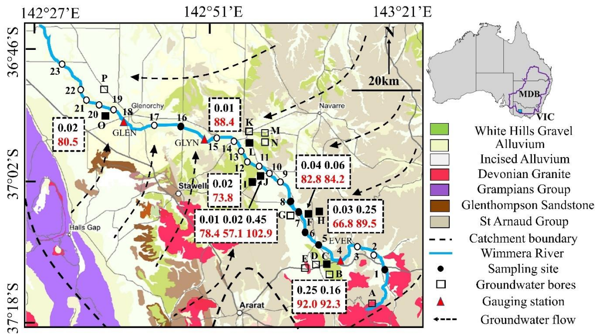
210 Figure 1. Summary geological and hydrogeological map of the upper Wimmera River. Stream water sampling sites and groundwater bores are indicated by numbers and letters, respectively. The sites that have radioactive isotope data are shown in solid symbols. Gauging stations with site number are Eversley (EVER; 415207), Glynwylln (GLYN; 415206), and Glenorchy (GLEN; 415201). Background geological map from Department of Jobs, Precincts and Regions (2021) (© State Government of Victoria 1996-2021); other 215 information from Robinson et al. (2006), Department of Environment, Land, Water and Planning (2021),
