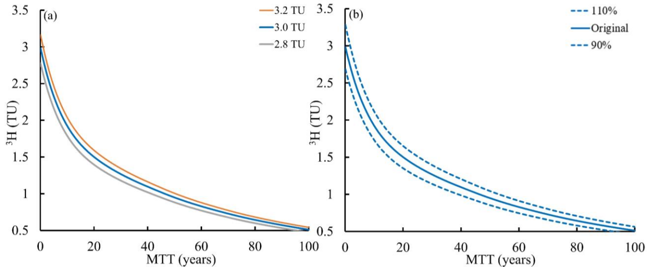
Figure 8. (a) Impacts of varying the 3 H activity of modern rainfall from 2.8 to 3.2 TU on MTTs calculated using the Exponential-Piston Flow Model (EPM ratio = 0.33). (b) Impacts of varying 3 H activity of rainfall between 90% and 110% of its assumed values on mean transit time calculated using the Exponential-Piston Flow Model (EPM ratio = 0.33). 505
