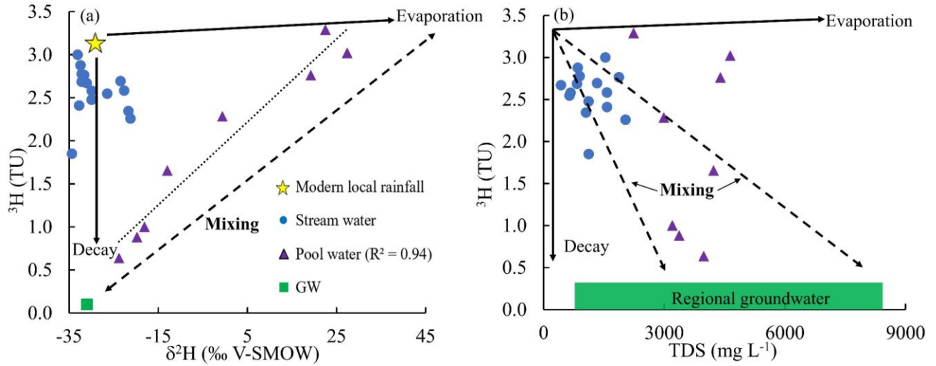
Figure 6. (a) Variation of 3 H activities and δ 2 H values and (b) 3 H activities and TDS of stream water, pool water and groundwater (GW) in the upper Wimmera catchment. arrows show trends expected from evaporation and mixing. Data from Table S1 and S2.
