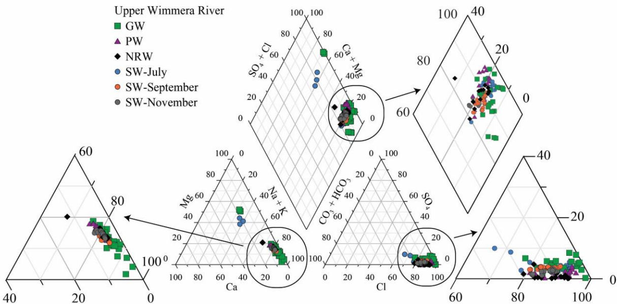
Figure 3. Trilinear diagram summarising molar major ion ratios of the different water sources in the upper Wimmera River (data from Table S1 and S2). GW=groundwater; PW= Pool Water; NRW=Near River Water; SW=Stream Water. Inserts show details of the data.
