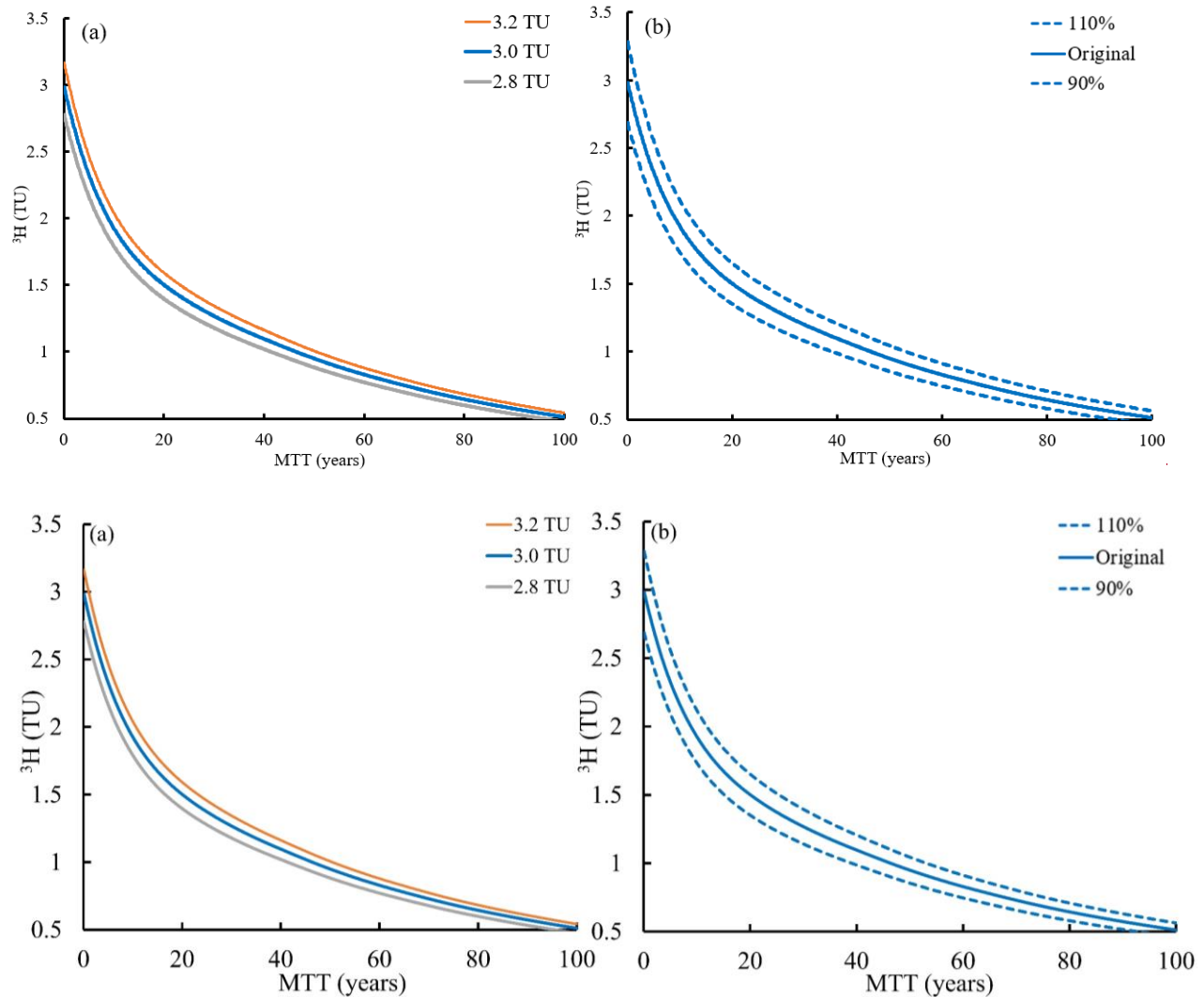
Figure 8. (a) Impacts of varying the ^3\text{H} activity of modern rainfall from 2.8 to 3.2 TU on MTTs calculated using the Exponential-Piston Flow Model (EPM ratio = 0.33). (b) Impacts of varying ^3\text{H} activity of rainfall between 90% and 110% of its assumed values on mean transit time calculated using the Exponential-Piston Flow Model (EPM ratio = 0.33).
