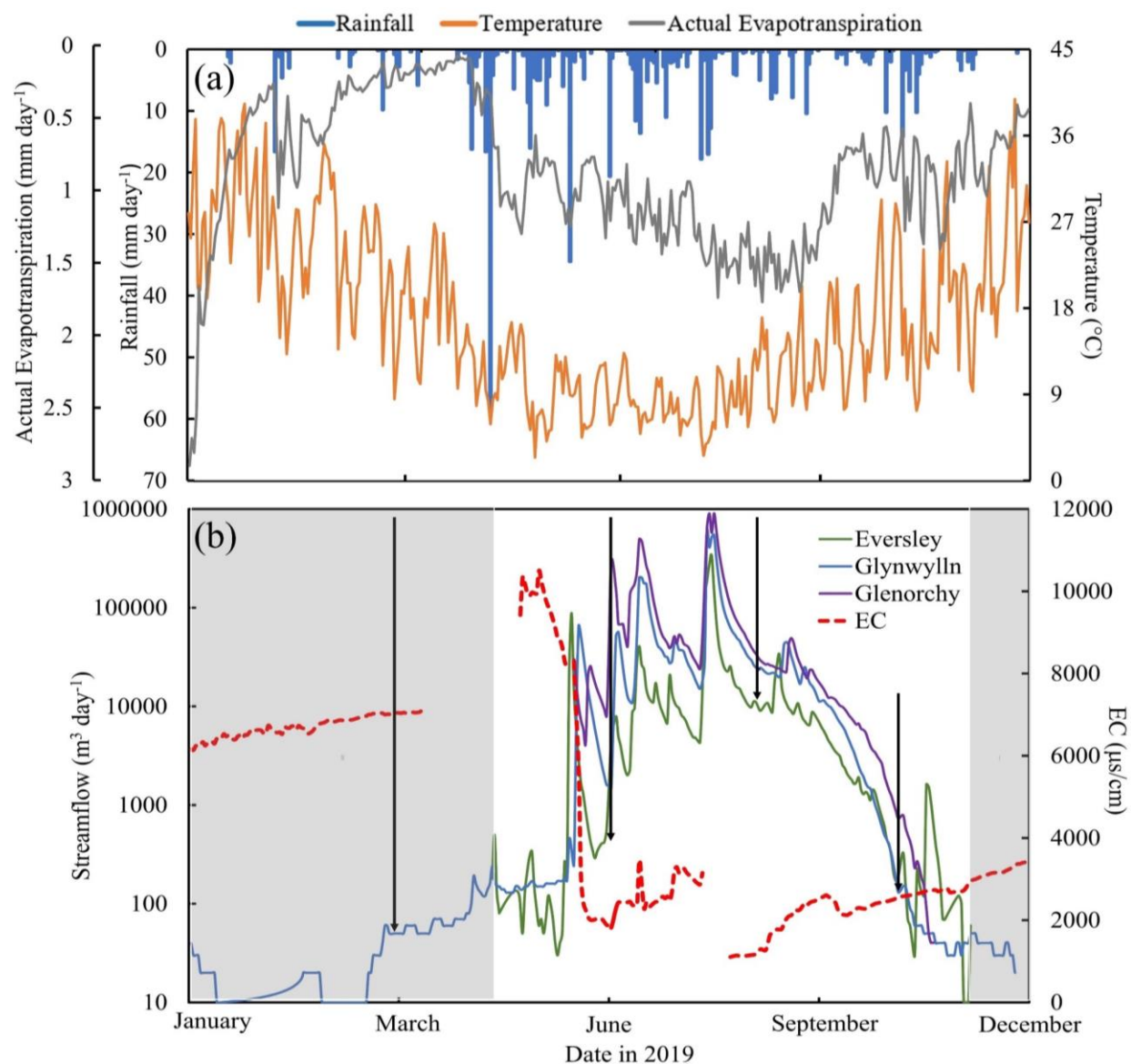
Figure 2. (a) Variations in daily rainfall, daily actual evapotranspiration , and temperature and (b) EC at Glynwylln (missing data are caused by measurement errors of equipment) and streamflow at Eversley, Glynwylln, and Glenorchy (Fig.1) in the upper Wimmera River in 2019. Variations in EC at Glynwylln (missing data are caused by measurement errors of equipment) and streamflow at Eversley, Glynwylln, and Glenorchy (Fig.1) in the upper Wimmera River in 2019. Sampling times are indicated by arrowed lines. Shaded areas represent the zero-flow periods. Data from Department of Environment, Land, Water and Planning (2021) and Bureau of Meteorology (2021).
