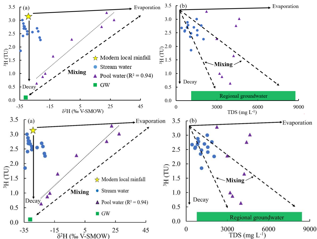
410 Figure 6. (a) Variation of ^3\text{H} activities and \delta^2\text{H} values and (b) ^3\text{H} activities and TDS of stream water, pool 415 water and groundwater (GW) in the upper Wimmera catchment. arrows show trends expected from evaporation and mixing. Data from Table S1 and S2.
