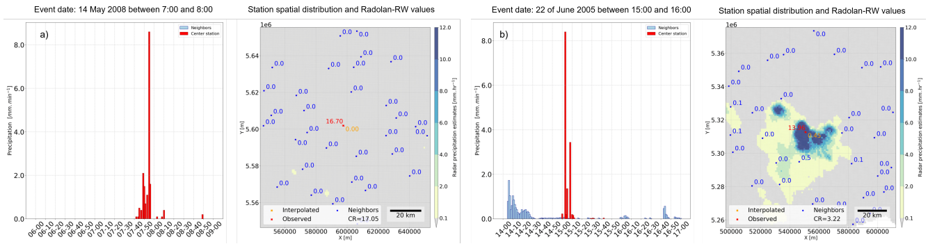
Figure 4. Panels a) and b) show two examples of an identified false observation and a single event in the minutely values that were verified using the Radolan-RW data. .
