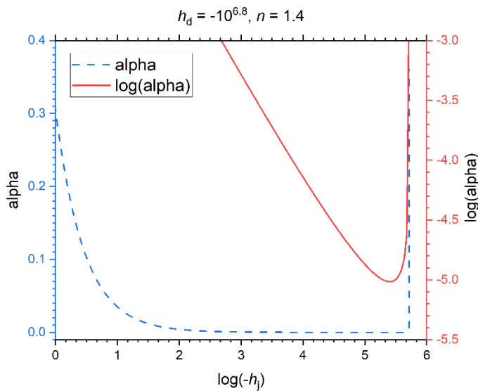
Figure 2: A transect of Figure 1 for n = 1.4 that shows the sharp increase of shape factor \alpha ( \text{cm}^{-1} ) as the matric potential at the junction point h_j ( \text{cm H}_2\text{O} ) reaches its physical limit defined in Eq. (4).
