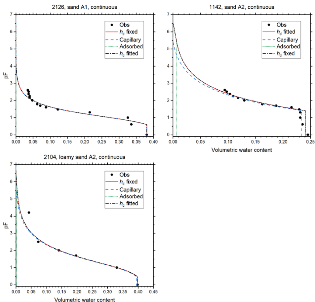
335 Figure 5: Soil water retention data and fitted curves for soils of classes A1 and A2 of Twarakavi et al. (2010). Curves fitted with h_d fixed at -10^{6.8} cm H_2O , and with h_d fitted with a cap at that value are shown. The one with the lowest Root Mean Square Error is shown in red. The volume fractions of capillary-bound water and water adsorbed in films is shown for this curve. The other curve is shown as black dash-dot line. This curve has not been corrected for continuity at the junction point. The vertical axes denote the logarithm (base 10) of the absolute value of the matric potential in cm H_2O .
