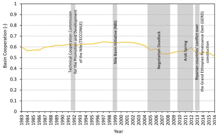
Figure 7: Simulated cooperation in the ENB (BC) with independent information on key events from 1983 to 2016.
