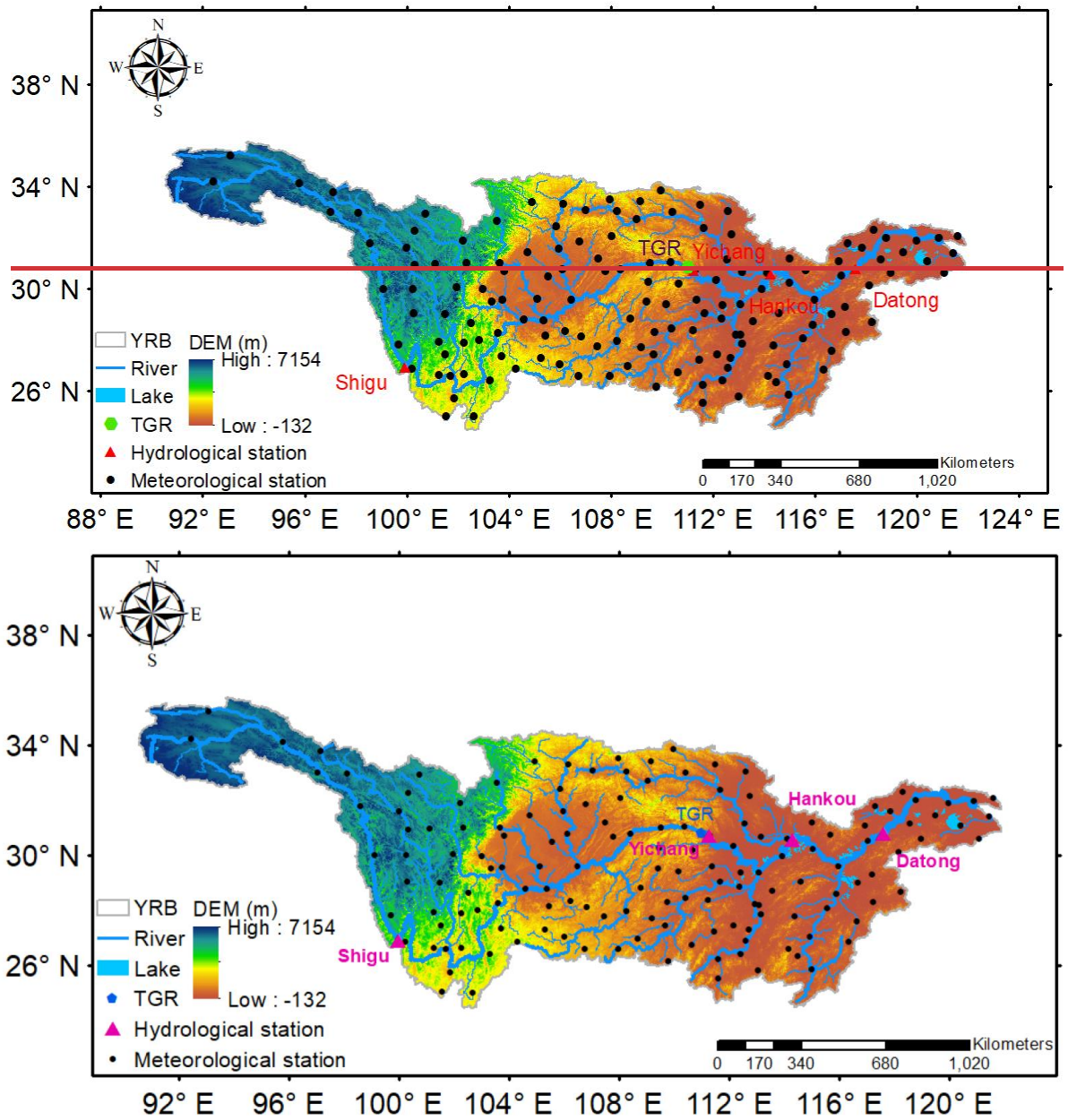
Figure 1: Location of the Yangtze River Basin (YRB) in China and its topography. Distribution of meteorological stations and hydrological stations are also shown in this figure. TGR = Three Gorges Reservoir; DEM = Digital Elevation Model.
