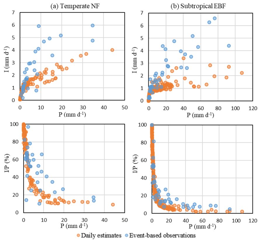
Figure S5. Comparisons between daily estimated interception with event-based observations from two field campaigns. The left column corresponds to a temperate NF in USA (Link et al., 2004), and the right column corresponds to a subtropical EBF in China (Chen and Li, 2016).
