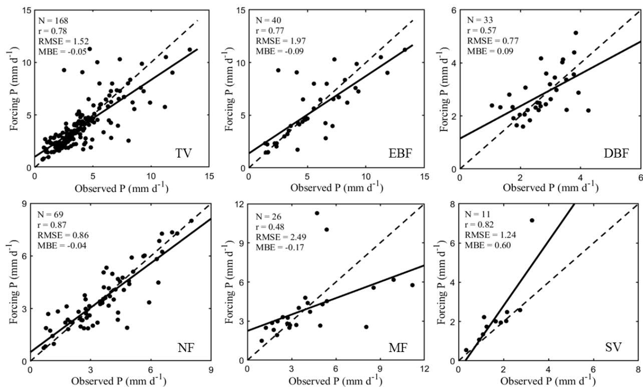
Figure S4. Linear regression between forcing and observed precipitation over field campaigns.
