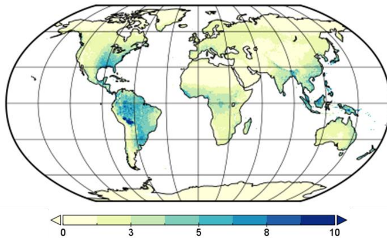
Figure S6. Global distribution of annual average rainfall rates ( \text{mm hr}^{-1} ) for 1980-2019.
