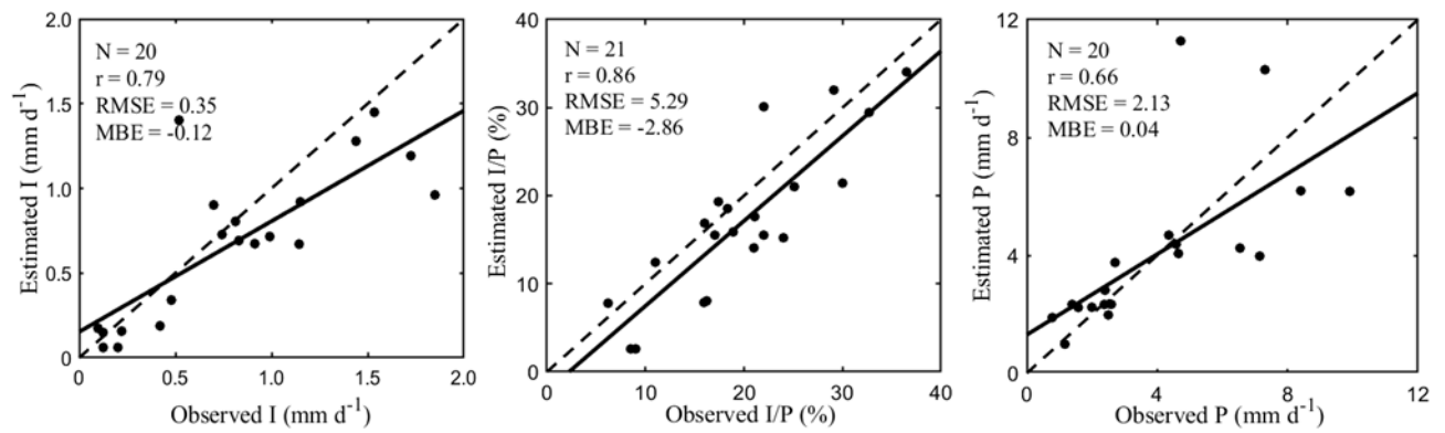
Figure S2. Field validation over marine forests. The black solid line represents the regression line, and the black dash marks the 1-to-1 line.
