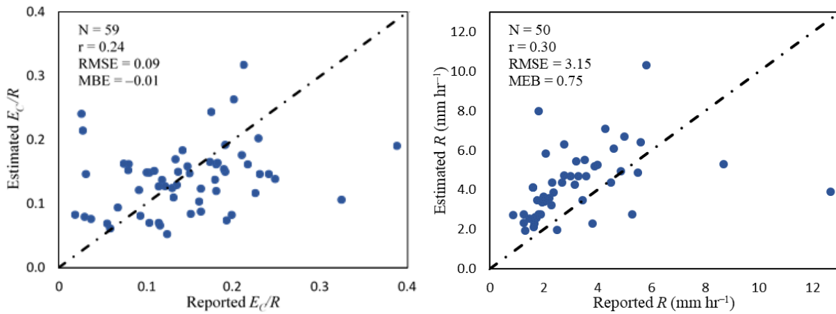
Figure S8. Comparison of tall vegetation E_c/R and R from publications and this study.
