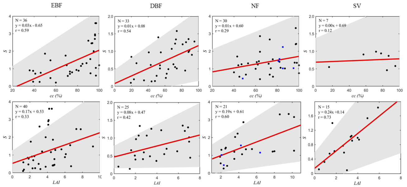
Figure S1. Linear regression between S and LAI , cc . The red line is the regression line, and the grey shading represents the 95% confidence interval. The blue scatters in NF represent the few values collected from MF.
