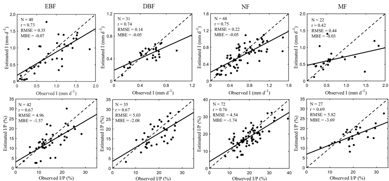
Figure S3. Field validation over different vegetation types. The black solid line represents the regression line, and the black dash marks the 1-to-1 line.
