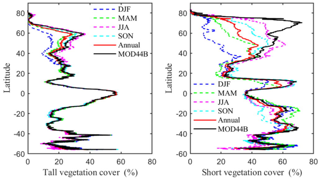
Figure S7. Variation of cc along different latitudinal bands. The dash lines represent the seasonal average (DJF: December–February; MAM: March–May; JJA: June–August; SON: September–November). The red solid line is the annual cc derived in this study, and the black solid line represents the annual cc from MOD44B product.
