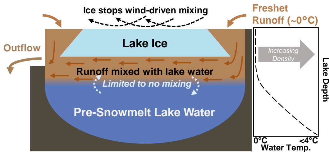
Figure 1. A conceptual cross-section of a an open-drainage lake when freshet has begun. Freshet initially flows into the lake at the edge where lake ice has melted. A layer of snowmelt runoff mixed with lake water then remains buoyant on top of the warmer lake water, before flowing through the outlet (i.e., ‘snowmelt bypass’). Limited mixing occurs due to density differences between runoff and deeper lake water, and the lack of wind-driven mixing due to the presence of lake ice.
