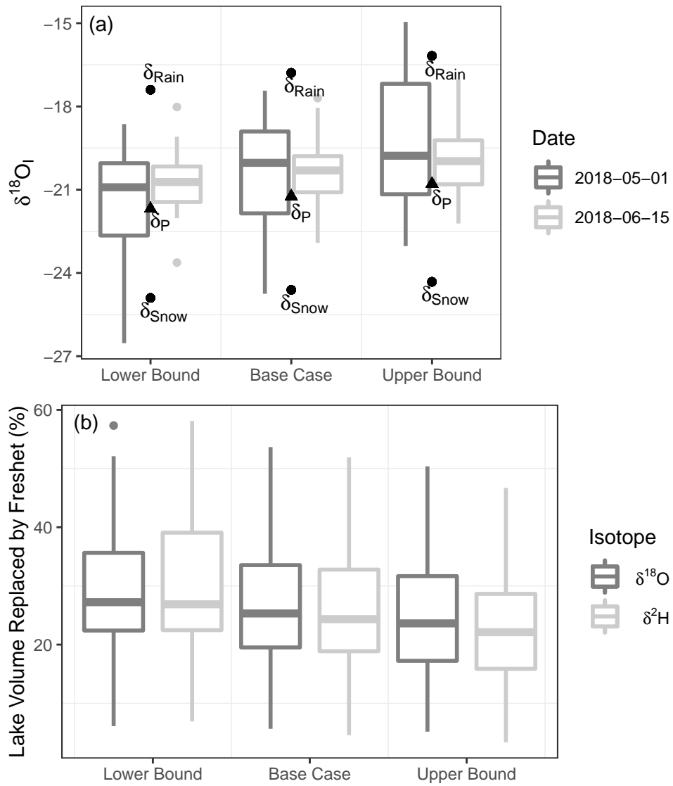
Figure B1. Comparison of upper and lower bound \delta_l and % lake water replacement values against the base case.
