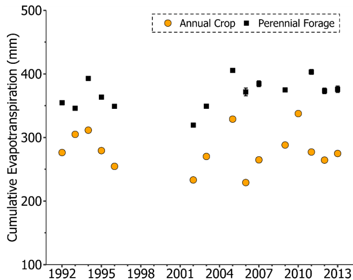
315 Figure 9: Comparison of annual cumulative evapotranspiration (ET) between annual crop and forage simulations at the La Salle River subbasin (LS-05OG008). The years 1997-2001, 2004, and 2008 were not used for model assessment due to missing data or equipment malfunctions.
