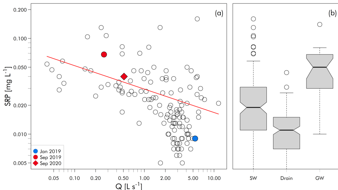
475 Figure 7: Long-term distribution of concentration discharge relationships for stream SRP at the catchment outlet (left), Box-Whisker plots of concentrations in stream water (SW, n=146), tile drains (Drain, n=138), and groundwater (GW, n=25) (right). Data are from Kistner (2007) (Drain), Dupas et al. (2017b) (SW), and UFZ TERENO monitoring, unpublished (GW) (see Supplement).
