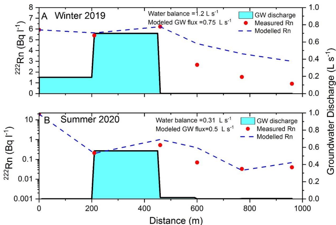
Figure 6: ^{222}\text{Rn} Radon concentrations in the stream water (measured and modelled) and groundwater discharge levels during A the winter (Jan. 2019) campaign and B the summer (Sep. 2020) campaign; groundwater discharge during the winter campaign includes drain water discharge; note that the most upstream “summer” sample was not considered representative of stream water (see Figure 5)
