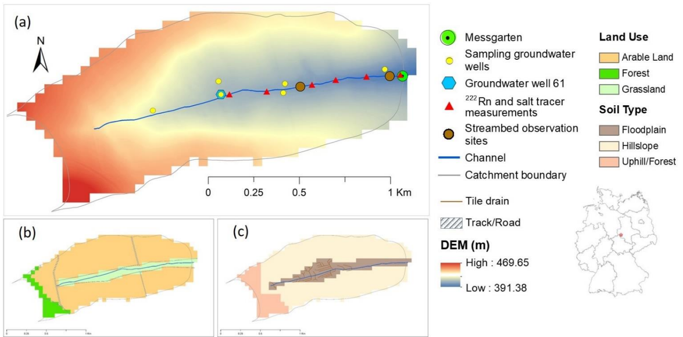
Figure 1. The Schäferal catchment and monitoring locations used by Yang et al. (2021), showing (a) digital elevation model (DEM) and monitoring sites with sampled groundwater wells, (b) land use types, and (c) soil types and the tile drain network. A V-notch weir is installed in the “Messgarten” climate station for discharge measuring and stream water sampling (adapted from Yang et al., 2021)
