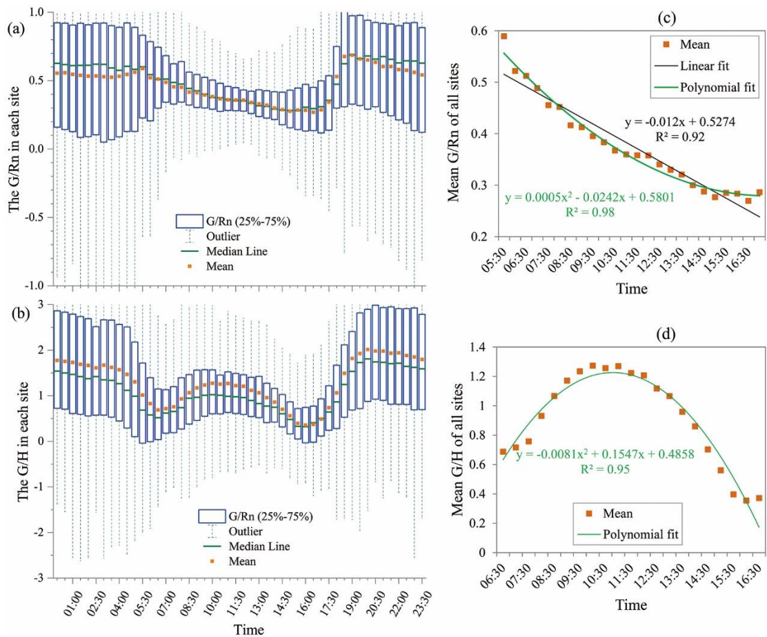
Figure 2: Intra-day distribution of the ratio of G and Rn (G/Rn) and the ratio of G and H (G/H) in each site (a and b are intra-day distributions of G/Rn and G/H ratios in each site, respectively; c and d are the fitted lines of the mean value of G/Rn and G/H in the daytime, respectively).
