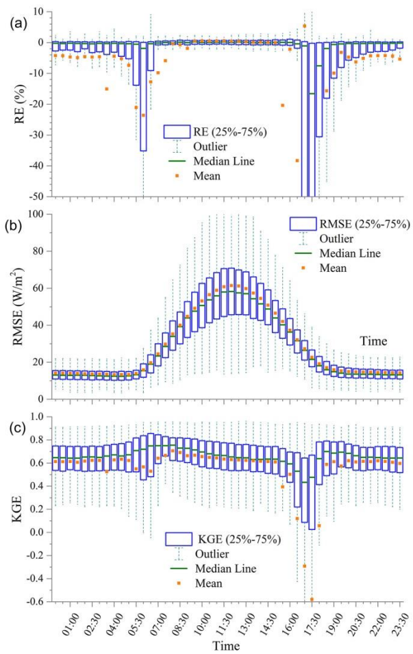
780 Figure 5: The RE, RMSE and KGE simulated by the LC method in each site and half-hour intervals.
