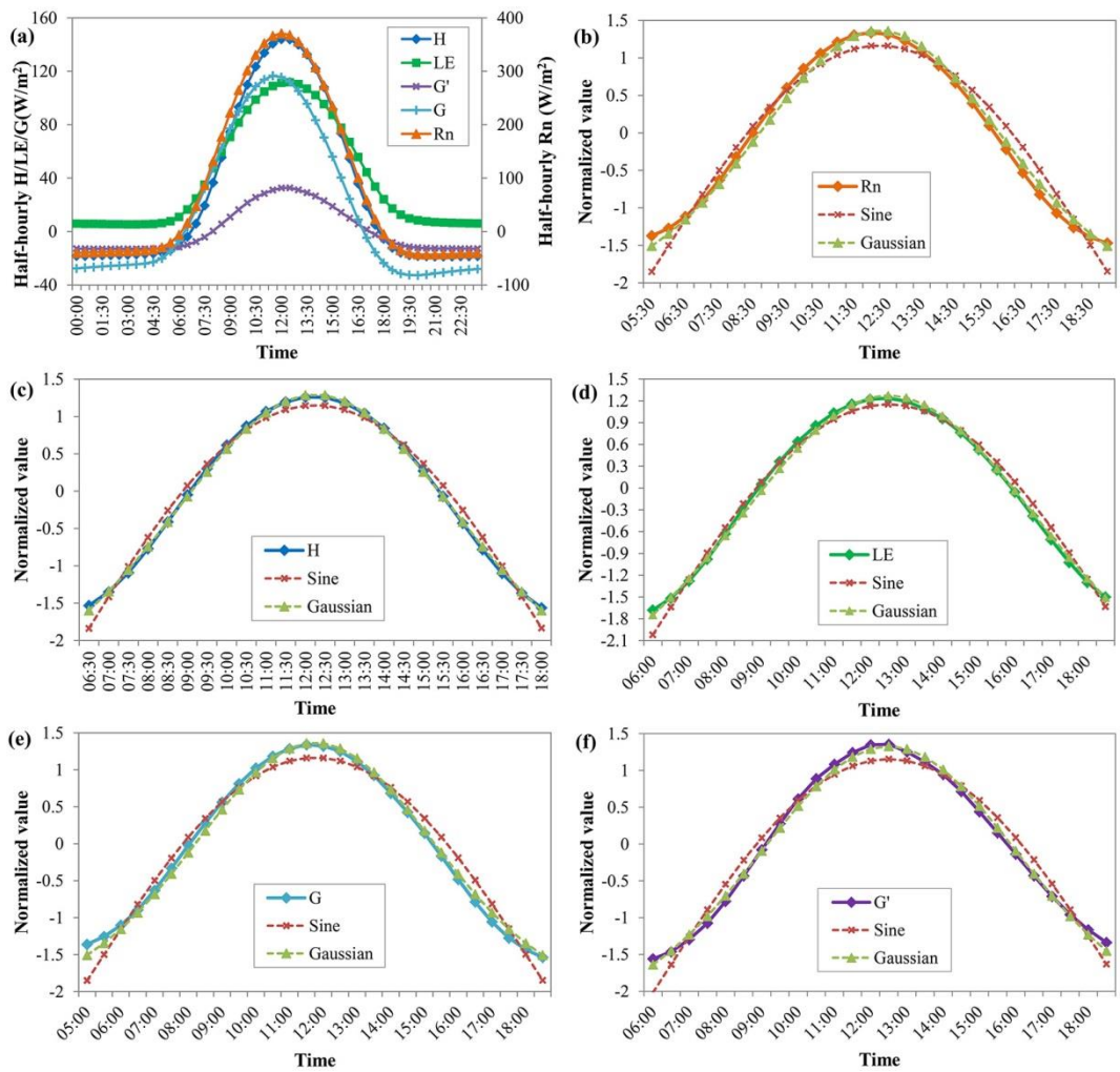
765 | Figure 1: Intra-day distribution of raw and normalized Rn, H, LE, G, G', and the values from the Sine and Gaussian functions (a is raw Rn, H, LE, G, and G'; b-f are normalized Rn, H, LE, G, and G', respectively).
