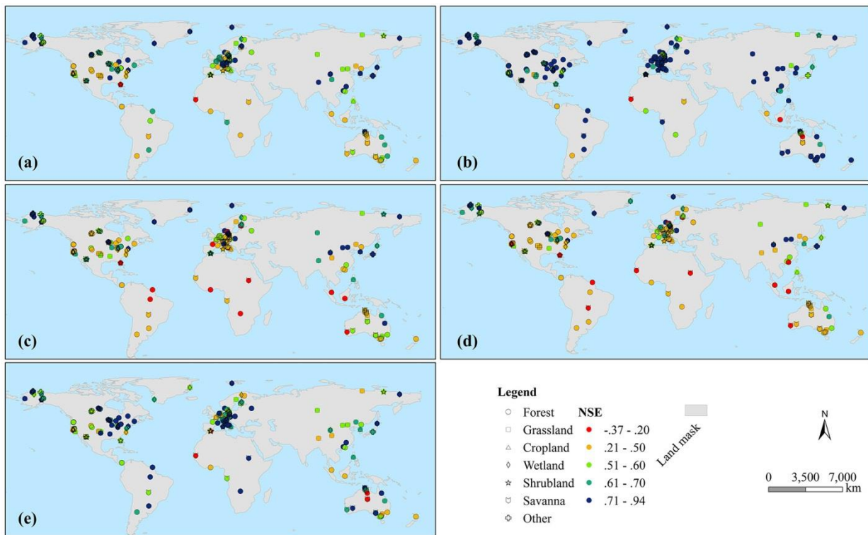
Figure 8: Spatial distribution of NSE values simulated by the LC method ( a is the median NSE of 48 half-hour values; ab-e represent the median NSE of half-hour values at 6:30, 10:30, 13:30 and 18:00, respectively).
