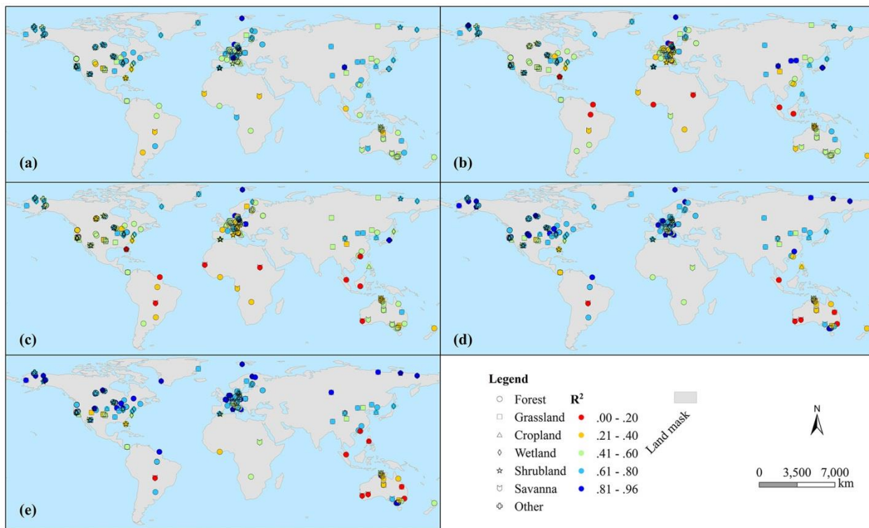
Figure 4: The linear or exponential fitting R^2 between daily series of G and Rn, and that between monthly series of G/Rn and NDVI at each observed site (a is the median R^2 of 48 half-hour periods at each site; b and c are the R^2 values between G and Rn at 10:30 and 13:30 respectively; d and e are linear and exponential functions fitting R^2 between G/Rn and NDVI, respectively).
