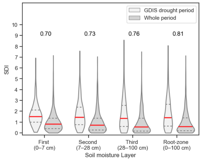
Figure 4: Comparison of SDI between the GDIS drought period and the whole period. The red line shows the median value and grey dotted lines show the 25th and 75th percentile values of each distribution. The value above the violin plot shows the difference of the median values in the GDIS drought period and the whole period.
