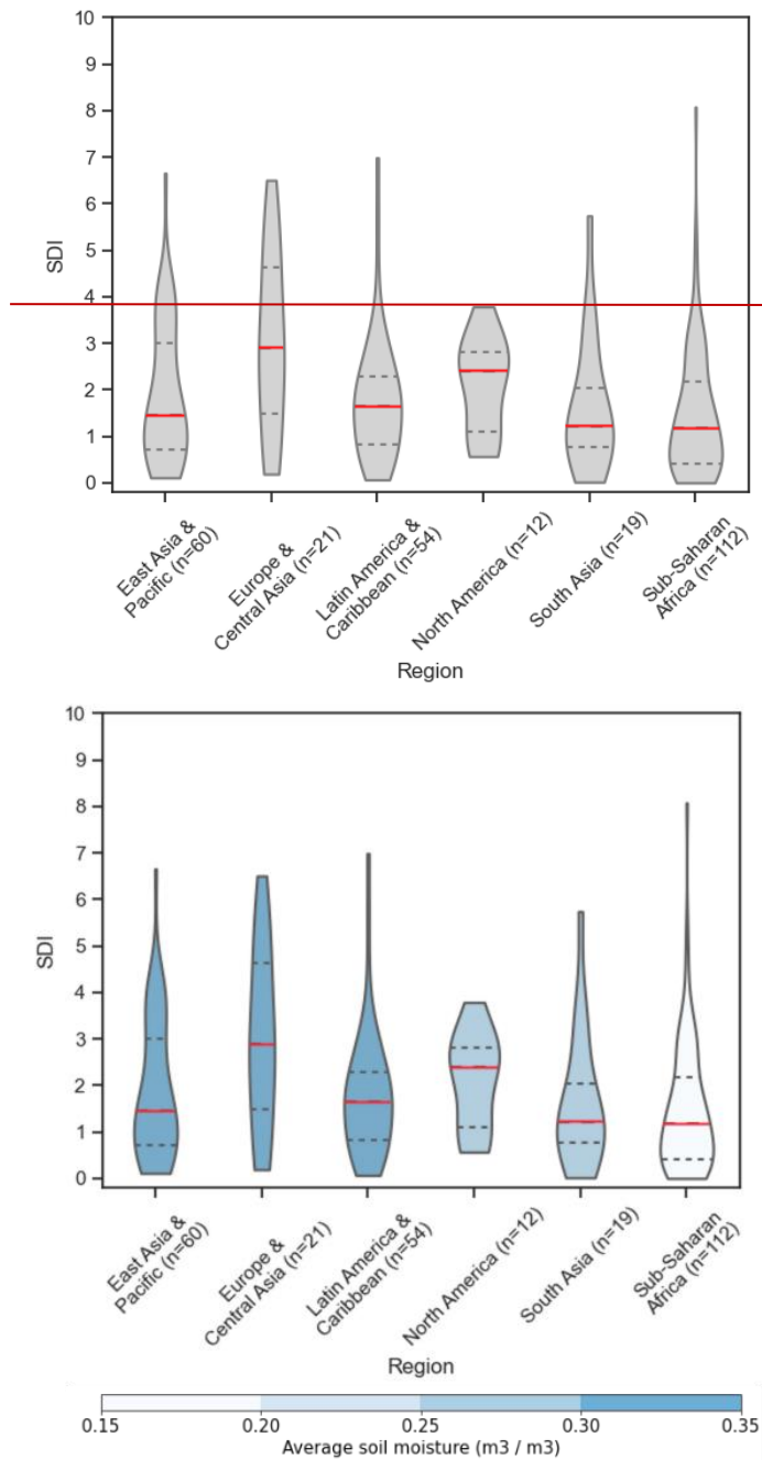
Figure 5: Comparison of the root-zone SDI by geographical regions. The red line shows the median value and grey dotted lines show the 25th and 75th percentile values of each distribution. The colour shows the average soil moisture over the study period (1964– 2018).
