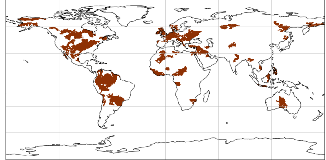
(b) Drought clusters
