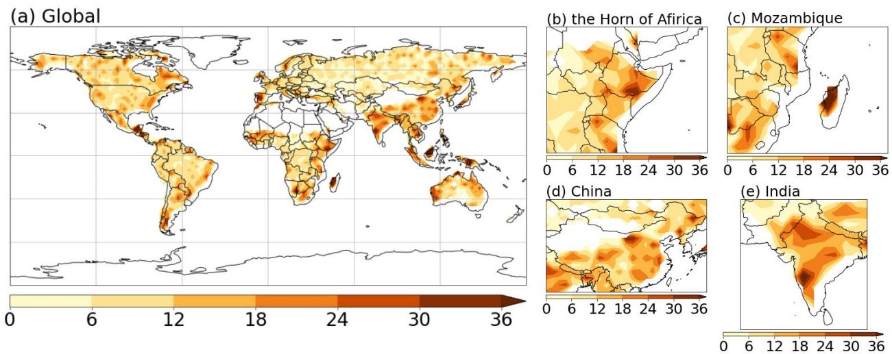
Figure 8: The number of drought cluster centroids based on ERA5-Land. (a) Global map, enlarged view of (b) the Horn of Africa, (c) Mozambique, (d) China, and (e) India.
