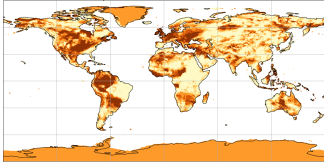
(a) Soil moisture percentile
