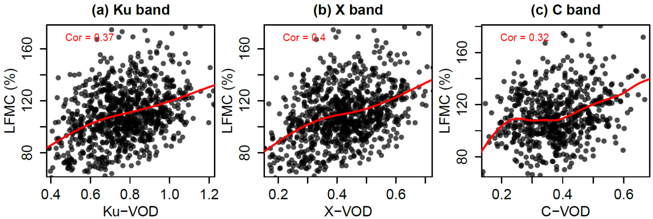
440 Figure 2: Global scatterplots and correlation of LFM C from the Globe-LFMC database against Ku-, X- and C-VOD. The red lines are smoothing spline fits between the values at the x- and y-axes.
