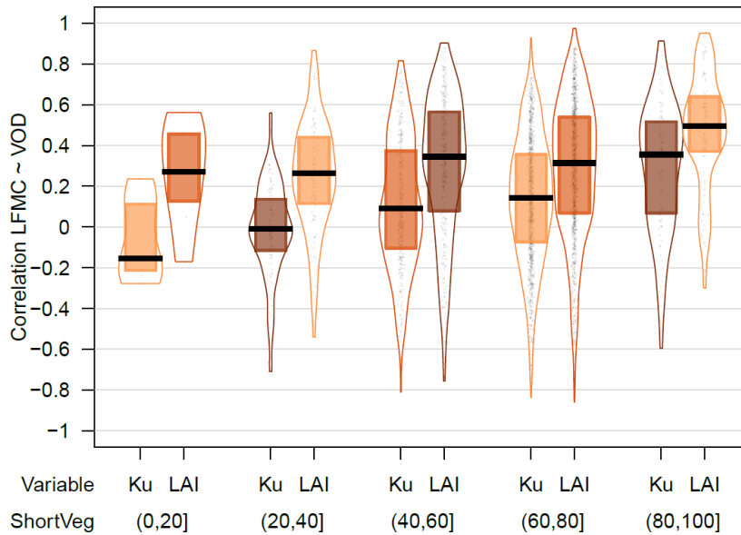
885 Figure A 5: Statistical distributions of the temporal correlation between Ku-VOD or LAI and measurements from the Globe-LFMC database stratified by the percentage cover of short vegetation.
