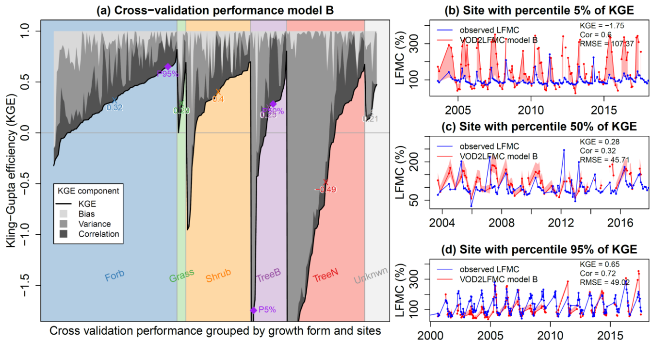
605 Figure 7: Performance of model B using Ku-VOD in spatial cross validation at each site grouped by the sampled vegetation growth form of LFM C measurements. (a) Kling-Gupta efficiency with its components caused by bias, variance and correlation. Purple dots represent the 5%, 50% and 95%-iles of the KGE across all sites. The time series of the sites corresponding to those percentiles are shown in panels (b, 5% = site with low performance, broad-leaved tree site), (c, 50% = site with medium performance, broad-leaved tree site) and (d, 95% = site with -good performance, forb site).
