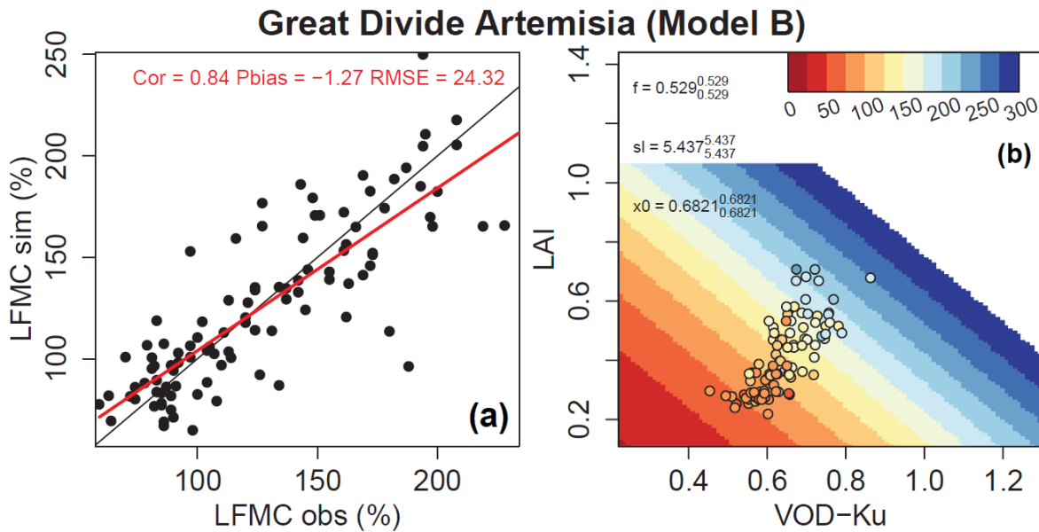
525 Figure 4: Example of the fit of model B using daily Ku-VOD and monthly LAI for Artemisia tridentata ssp. at the site Great Divide, Colorado (40.76°N, 107.85°W). (a) Scatterplot of estimated against observed LFM C. (b) Distribution of observed LFM C (points) and estimated LFM C (coloured background) in relation to daily Ku-VOD and monthly LAI.
