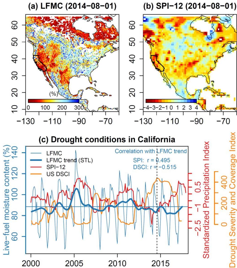
770 Figure 10: Comparison of LFMF as estimated from model B with drought conditions in North America and California. (a) Map of mean monthly LFMF for August 2014, a month with severe drought in the western United States. The state of California is highlighted in the map. (b) Map of the Standardized Precipitation Index for 12-monthly accumulation periods (SPI-12) for August 2014. SPI-12 data is taken from GDO (2021). (c) Comparison of LFMF, SPI-12 and the US Drought Severity and Coverage Index (DSCI) for California. A severe drought started in California (and in the western US) in 2013 and lasted until end 2016 as shown by negative SPI-12 values, very high DSCI values, and low LFMF. The dashed vertical line corresponds to August 2014, which is shown as map in panels (a) and (b).
