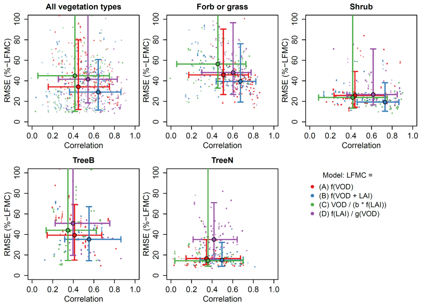
560 Figure 5: Performance of the models A-D using daily Ku-VOD (and monthly LAI in models C-D) after calibrating each model at each site. Shown is the root mean squared error (RMSE) and correlation coefficient between estimated and measured LFMC. Small dots are results from different parameter sets at each site, big dots and bars are the median and range from the 5 to 95%-iles across all sites, respectively.
