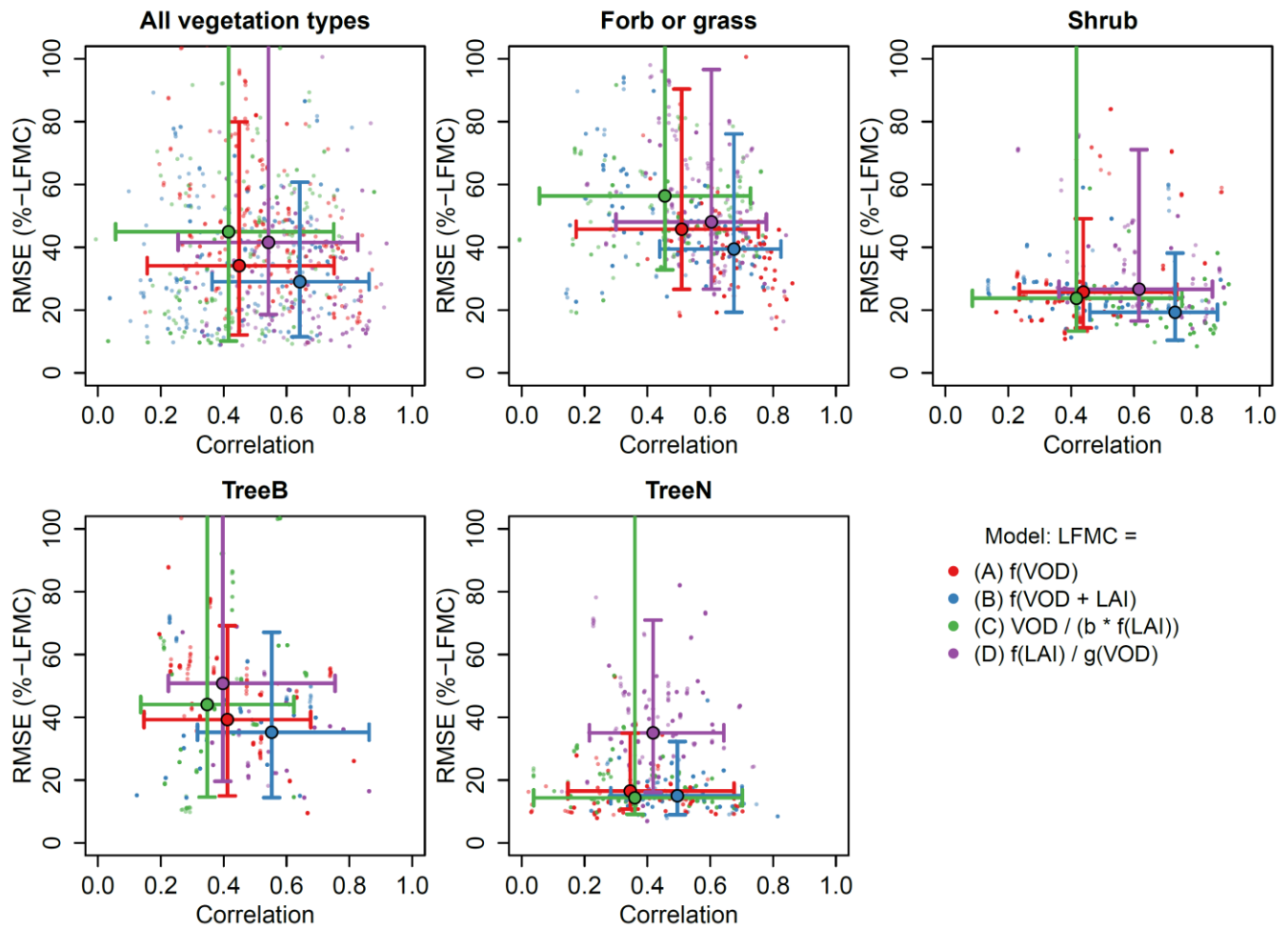
550 Figure 5: Performance of the models A-D using daily Ku-VOD (and monthly LAI in models C-D) after calibrating each model at each site. Shown is the root mean squared error (RMSE) and correlation coefficient between estimated and measured LFMC. Small dots are results from different parameter sets at each site, big dots and bars are the median and range from the 5 to 95%-iles across all sites, respectively.
