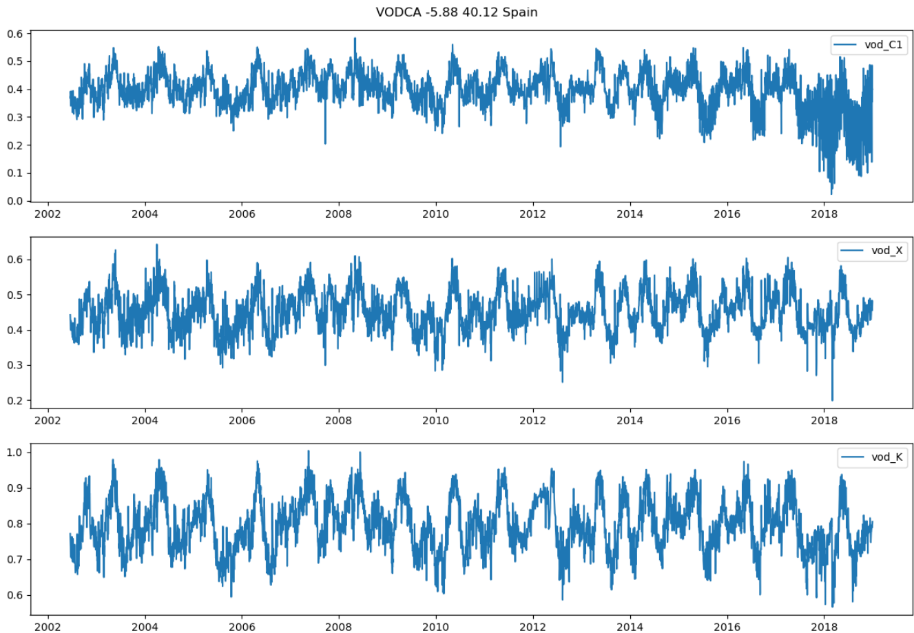
845 Figure A 1: Example time series of C-, X- and Ku-VOD over a grid cell in Spain (5.88°W, 40.12°N), where the C-VOD time series shows a high level of noise likely caused by RFI in the later years.
