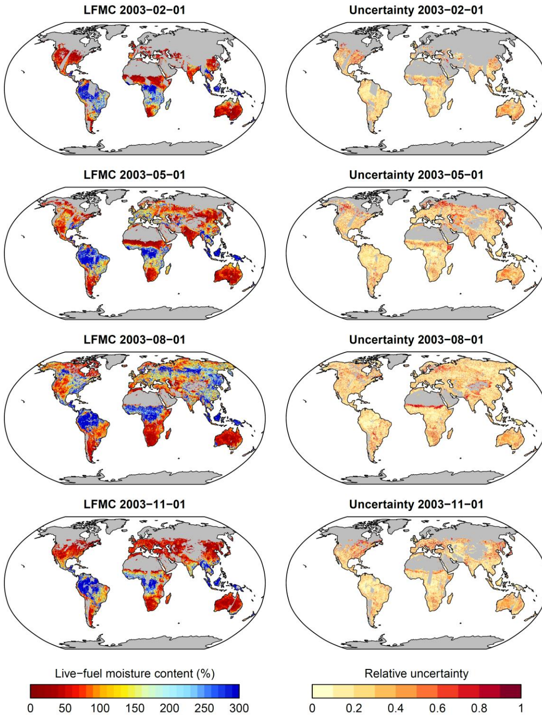
Figure 8: Example of global patterns of LFMC and associated uncertainties as estimated with model B for four selected days in 2003, representing typical days during the northern seasons and the wet and dry seasons in Africa. Grey areas (missing data) is because of missing vegetation cover or gaps in the LAI or VOD data.
