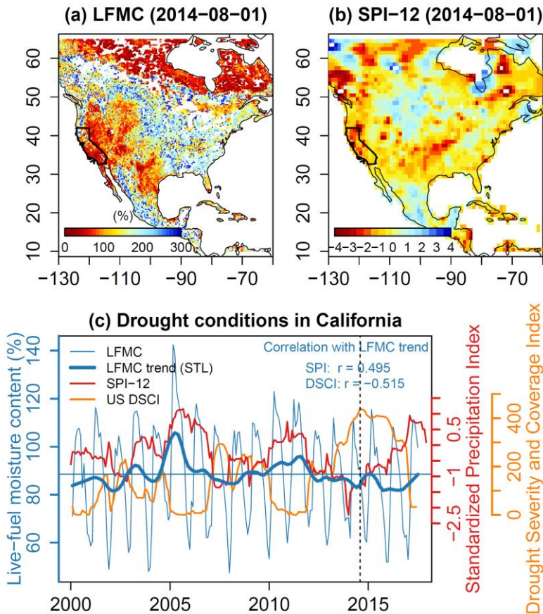
760 Figure 10: Comparison of LFMF as estimated from model B with drought conditions in North America and California. (a) Map of mean monthly LFMF for August 2014, a month with severe drought in the western United States. The state of California is highlighted in the map. (b) Map of the Standardized Precipitation Index for 12-monthly accumulation periods (SPI-12) for August 2014. SPI-12 data is taken from GDO (2021). (c) Comparison of LFMF, SPI-12 and the US Drought Severity and Coverage Index (DSCI) for California. A severe drought started in California (and in the western US) in 2013 and lasted until end 2016 as shown by negative SPI-12 values, very high DSCI values, and low LFMF. The dashed vertical line corresponds to August 2014, which is shown as map in panels (a) and (b).
