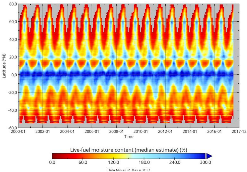
Figure 9: Hovmoeller diagram of monthly LFMC as estimated from model B using daily Ku-VOD and monthly LAI.
