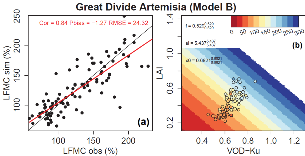
515 Figure 4: Example of the fit of model B using daily Ku-VOD and monthly LAI for Artemisia tridentata ssp. at the site Great Divide, Colorado (40.76°N, 107.85°W). (a) Scatterplot of estimated against observed LFM. (b) Distribution of observed LFM (points) and estimated LFM (coloured background) in relation to daily Ku-VOD and monthly LAI.
