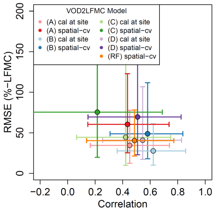
585 Figure 6: Performance of the models A-D using Ku-VOD after calibrating each model for each species at each site (cal at site) and after using sites as test data in spatial cross validation after the application of random forest to predict model parameters (spatial-cv). The global RF model (shown in orange) was directly trained against LFMC measurements from multiple sites. Shown is the root mean squared error (RMSE) and correlation coefficient between estimated and measured LFMC. Dots and bars are the median and range from the 5 to 95%-iles across all sites, respectively.
