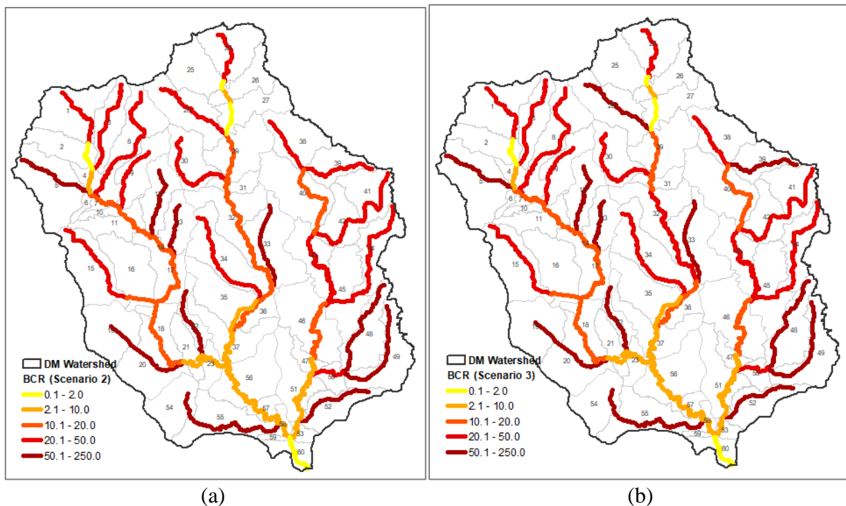
910 Figure 9. (a) Benefit-Cost Ratio map for full riparian restoration (Scenario 2). (b) Benefit-Cost Ratio map for efficient riparian restoration (Scenario 3). The reduction in the number of days that exceed 18 °C was considered a riparian restoration benefit. The cost corresponds to the 2010 riparian restoration cost in millions of dollars.
