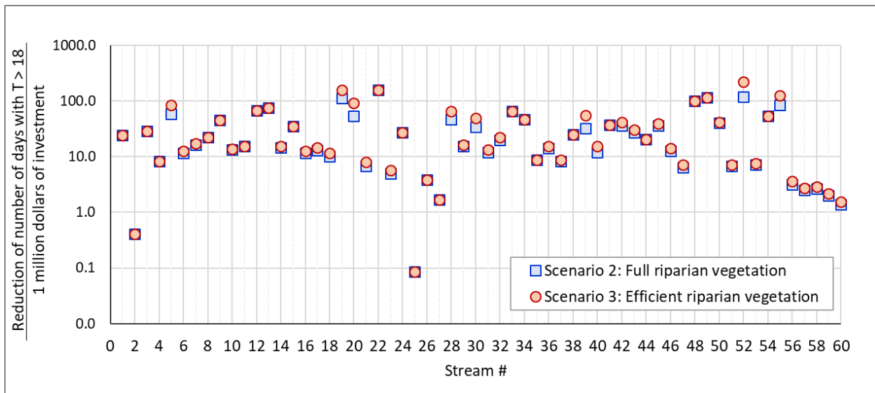
905 Figure 8. Benefit-Cost Ratio (Reduction of the number of days that exceed 18 °C / cost of the riparian restoration in millions of dollars) for the 60 DMW stream for the case of full riparian restoration (Scenario 2) and efficient riparian restoration (Scenario 3).
