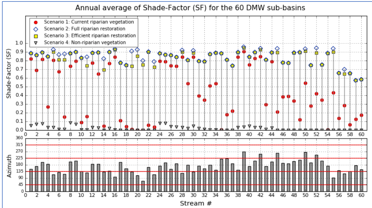
Figure 5. Annual average of Shade Factors (SF) for the 60 DMW streams for scenarios 1, 2, 3 and 4.
