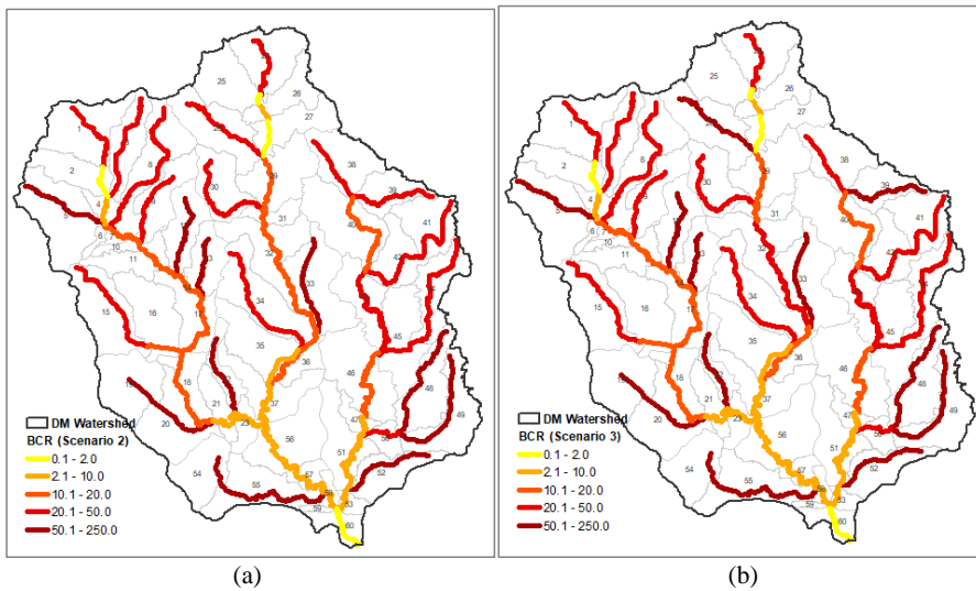
880 Figure 9. (a) Benefit-Cost Ratio map for full riparian restoration (Scenario 2). (b) Benefit-Cost Ratio map for efficient riparian restoration (Scenario 3). The reduction in the number of days that exceed 18 °C was considered a riparian restoration benefit. The cost corresponds to the 2010 riparian restoration cost in millions of dollars.
