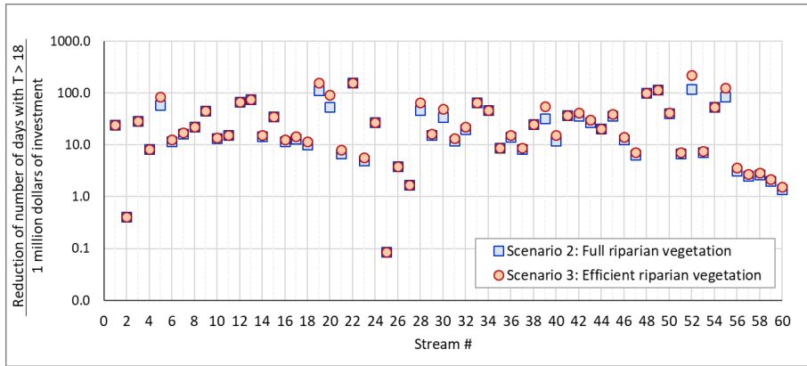
875 Figure 8. Benefit-Cost Ratio (Reduction of the number of days that exceed 18 °C / cost of the riparian restoration in millions of dollars) for the 60 DMW stream for the case of full riparian restoration (Scenario 2) and efficient riparian restoration (Scenario 3).
