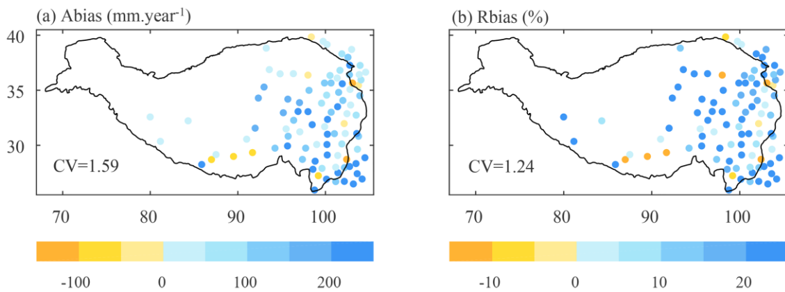
Figure 7 Spatial distribution of (a) absolute bias (Abias) and (b) relative bias (Rbias) for annual precipitation from ERA5_CNN during 1980-2018 at stations of China Meteorological Administration.
