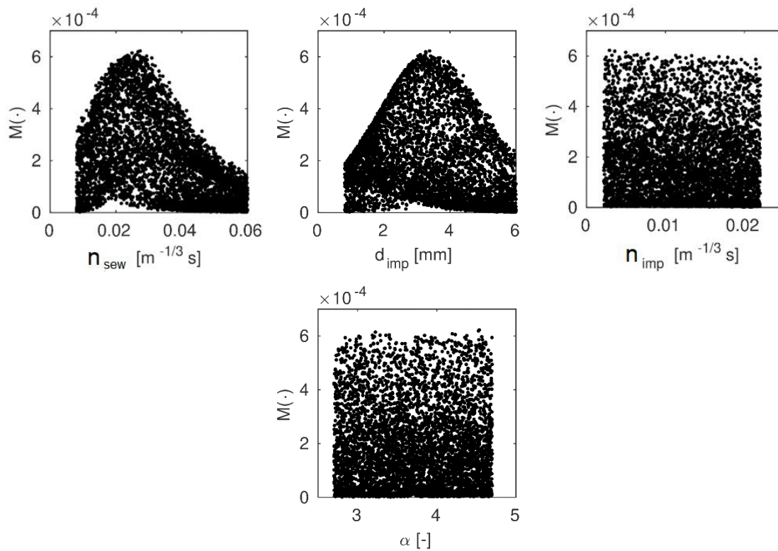
Figure B3. Calculated likelihood function — scatter plots of M values versus calibrated catchment parameters in SWMM.
