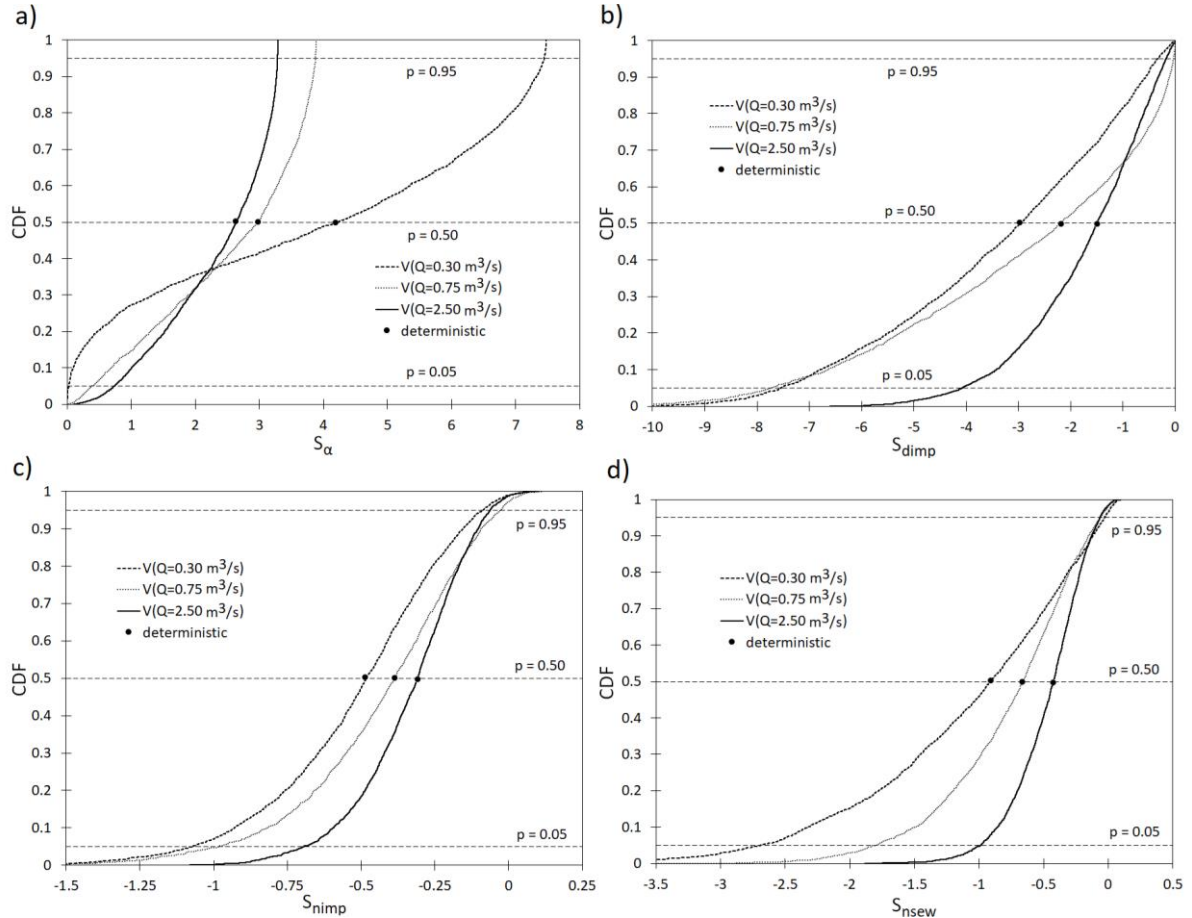
Figure 5: Comparison of calculation the calculated results (deterministic and probabilistic solutions) of sensitivity coefficients ( S_\alpha , S_{dimp} , S_{nimp} , and S_{nsew} ) for (a ÷ d) threshold values V(Q)=V_g and temporal rainfall distribution \xi=R1, R2 , and R3 .
