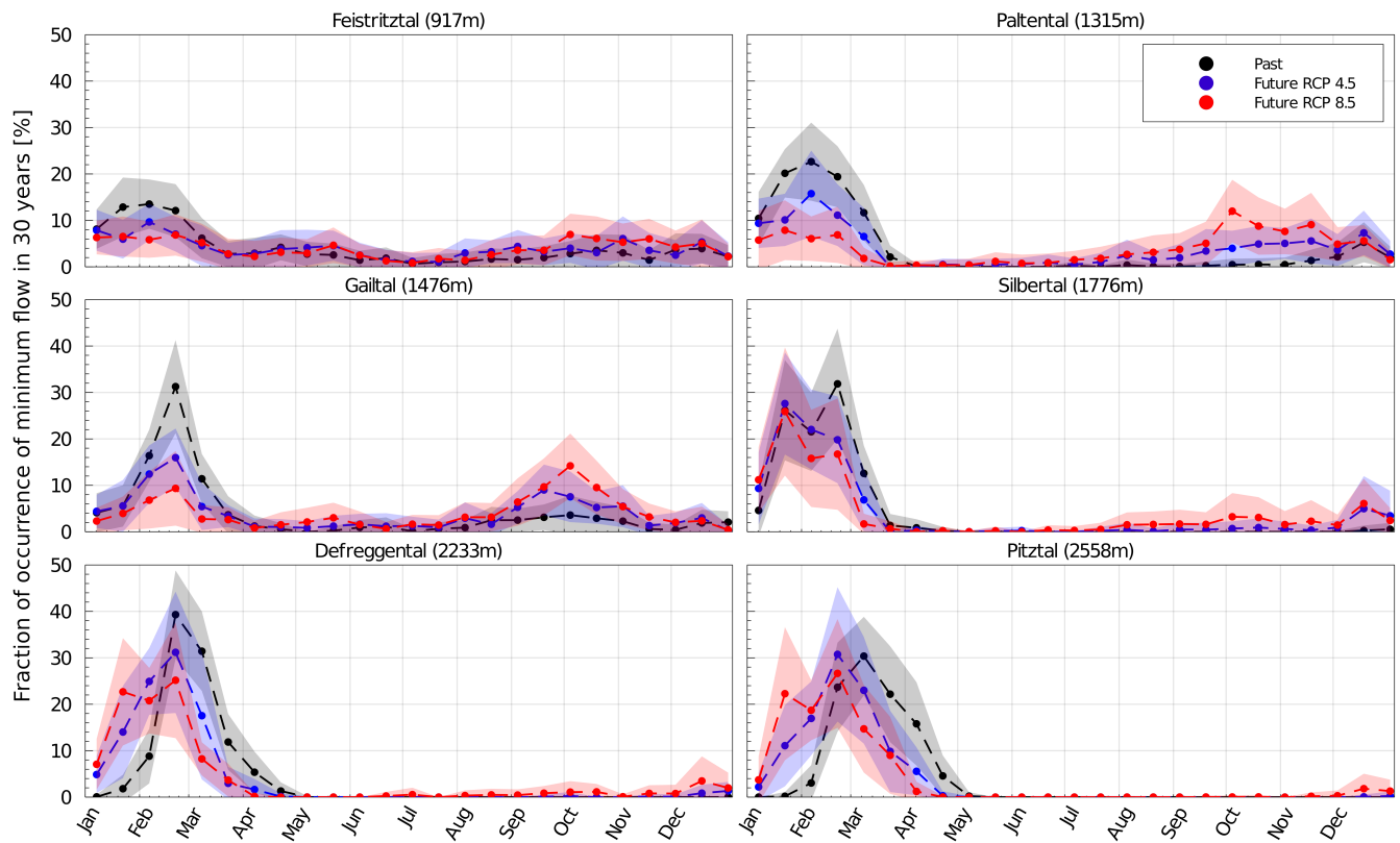
Figure 13. Mean fraction of occurrences of lowest annual 7-day flow in past (black symbols) and future (blue symbols: RCP4.5 RCP 4.5 , red symbols: RCP8.5 RCP 8.5 ) 30-year time periods using time windows of 15 days across all model simulations. The shaded areas indicate the associated \pm 1 standard deviation. Dashed lines between the individual 15-day periods are used for better visualization.
