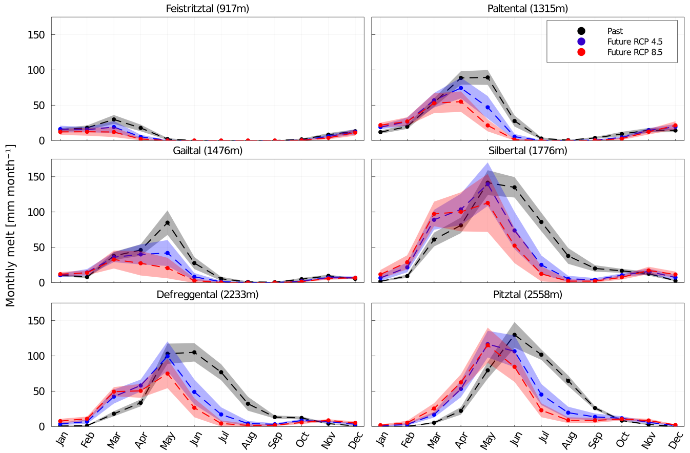
Figure 10. Mean monthly melt contributions in the past (black symbols) and future (blue symbols: RCP4.5 , red symbols: RCP8.5 ) over the time period of 30-years. The shaded areas indicate the associated \pm 1 standard deviations (grey: past, blue: RCP4.5 and red: RCP8.5 ). Dashed lines between the individual 15-day-periods-months are used for better visualization
