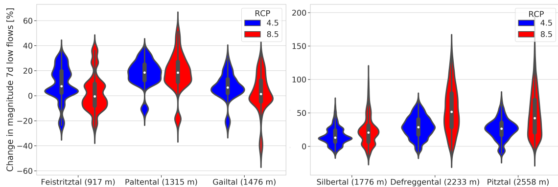
Figure 14. Relative change in magnitude of annual minimum 7-day flows for the late 21st 21st century (2071–2100 vs. 1981–2010). Note the different scales for low- and high-elevation catchments.
