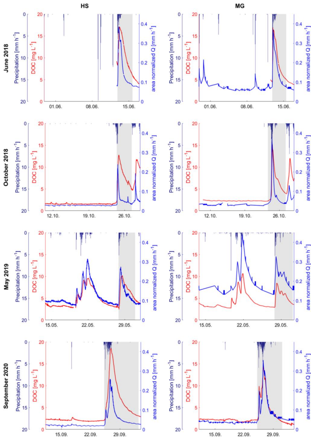
270 Figure 4: DOC concentrations and area normalized Q starting 14 days prior to the events in June 2018 (top row), October 2018 (second row), May 2019 (third row) and September 2020 (bottom row) at HS (left) and MG (right). The shaded areas highlight the events described in detail in Table 2.
