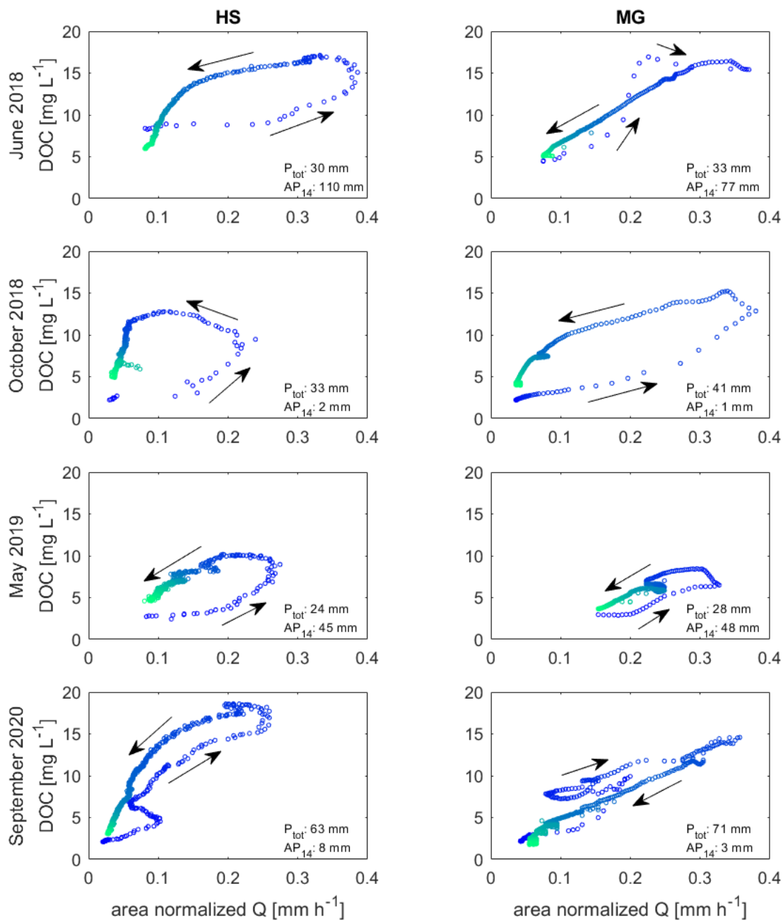
285 Figure 5: DOC-Q-Hysteresis during the events in June 2018, October 2018, May 2019 and September 2020 at HS and MG. The dots represent 15-minute time steps starting from dark blue to green and represent the events that are marked by the grey areas in Figure 45.
