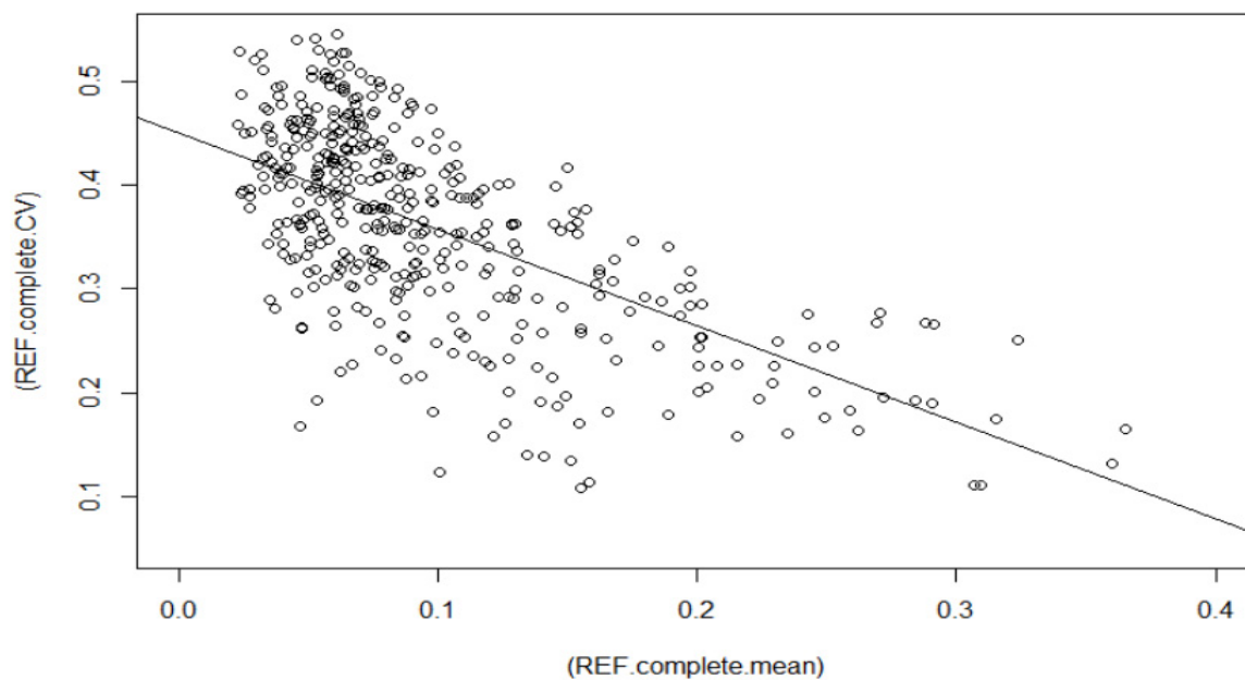
80 Figure S2: Coefficient of variation ( REF.complete.CV ) versus the mean normalized intensities ( REF.complete.mean ) of the common FT-ICR-MS reference samples compounds ( n = 422 ). Black line indicates linear regression. Mean REF.complete.CV was 0.36.
