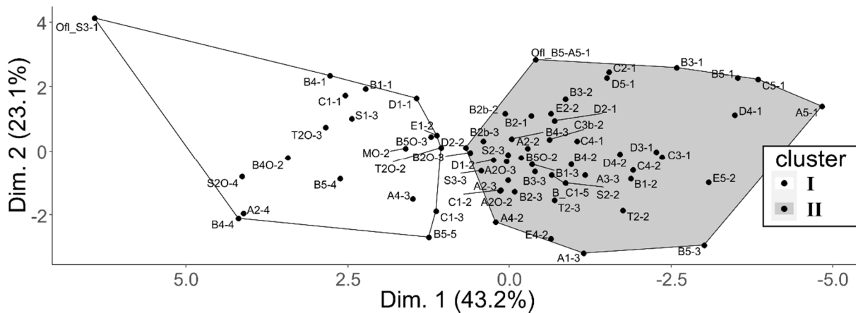
100 Figure S6: Visualization of the k-means cluster analysis on principal components for riparian samples only.
