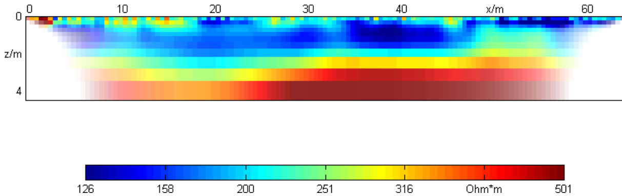
Figure S4: Electrical resistivity plot of the transect AB derived from geoelectrics.
