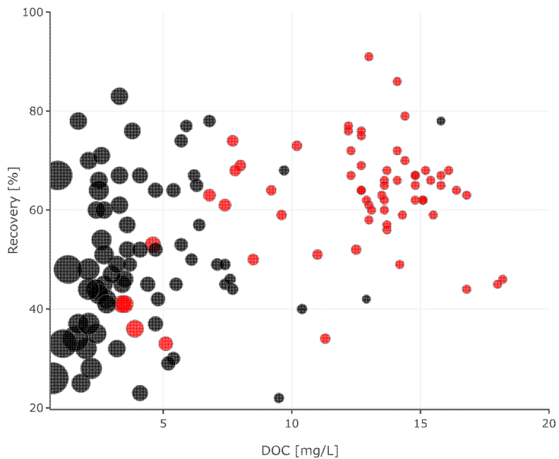
Figure S8: Quality control of solid phase extraction for DOC samples. SPE recovery vs sample DOC concentration for stream (red) and riparian samples (black) with dot size corresponding to the sample volume used for the extraction (range: 15-200 mL, n = 133 ).
