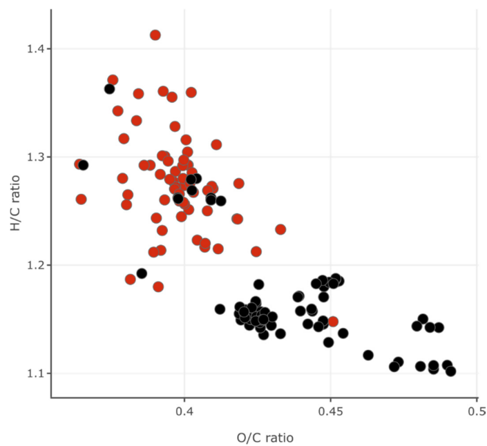
Figure S10: Aggregated van Krevelen plot of all FT-ICR-MS sample of stream (red) and riparian (black) origin. Data represent the intensity weighted average of the molecular H/C and O/C ratios considering all valid MF in these samples.
