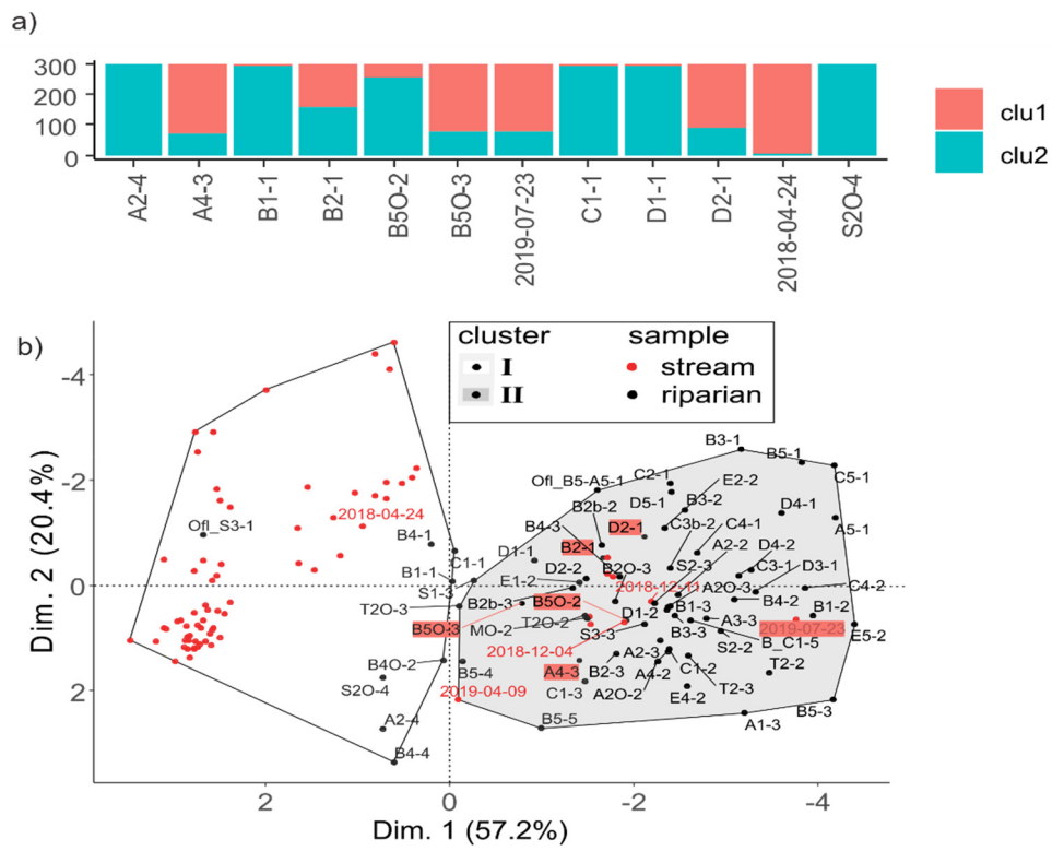
Figure S3: a) Bootstrapping of cluster analysis. Only samples are depicted where the random deviation made samples switch between the two clusters. Overall there are 143 samples. b) Visualization of k-means clustering results of all samples. Highlighted samples in red indicate samples with a probability of p > 0.05 to switch between clusters (see (a)). Samples marked with red dates indicate stream water samples of riparian sampling dates.
