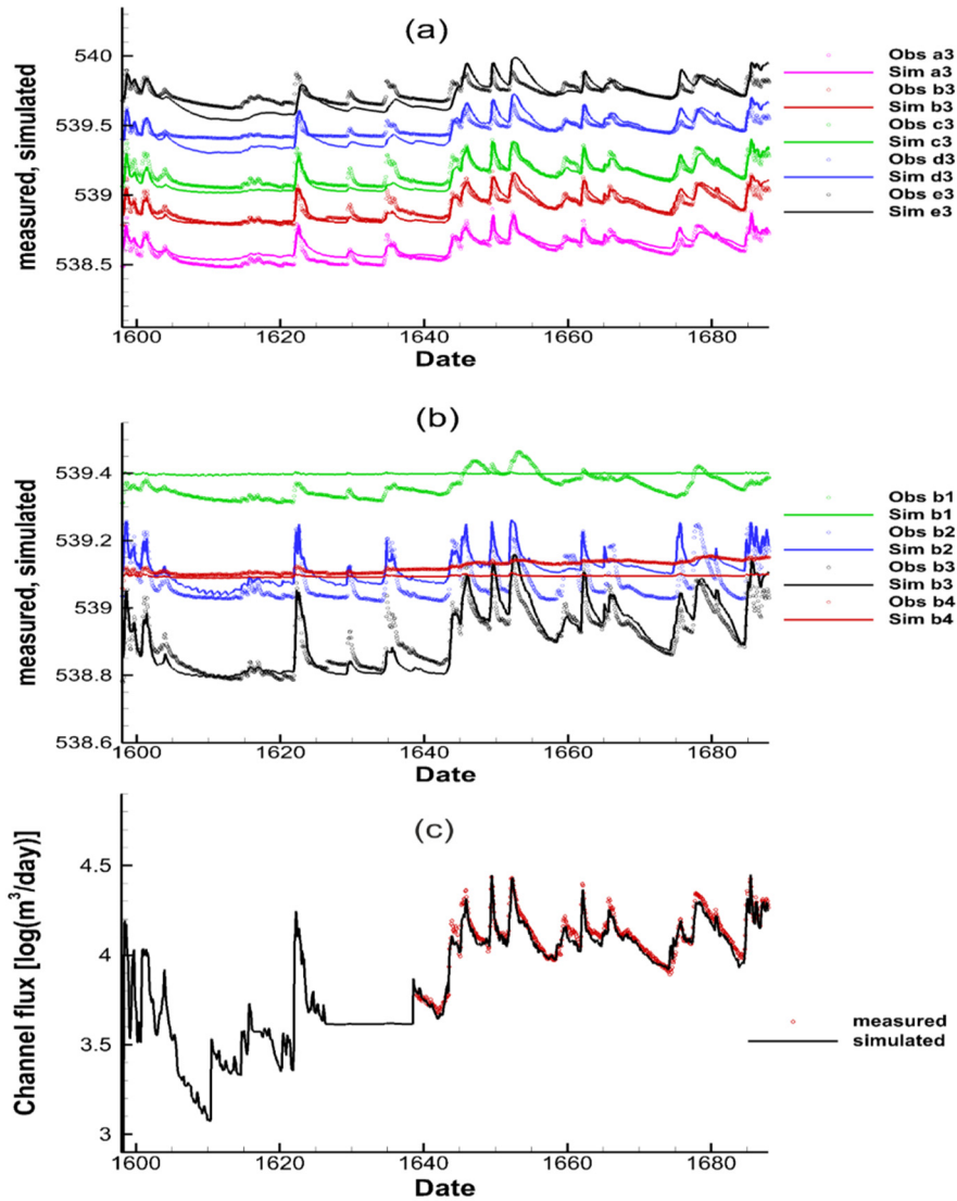
95 Figure S5: Comparison between the simulated groundwater levels and the measured ones for (a) five wells close to the channel, and for (b) wells along cross-section B, with the well b2 and b3 closer to channel, and b1 and b4 close to side boundaries. (c) Comparison between the simulated and the measured channel fluxes at the outlet.
