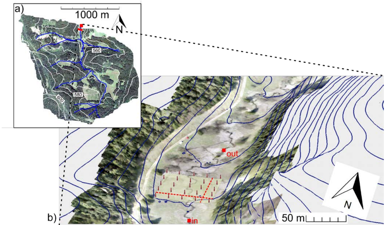
130 Figure 1. a) Rappbode catchment and position of the study site (red square). b) 3D view of the study site (red squares indicate in and outlet stream gauges). Red pins indicate the soil sampling transect and the piezometer network. Location of electric resistivity tomography indicated by red dashed lines. Note the 2.5-fold vertical exaggeration. Map data: ©Google, GeoBasis-DE-BKG.
