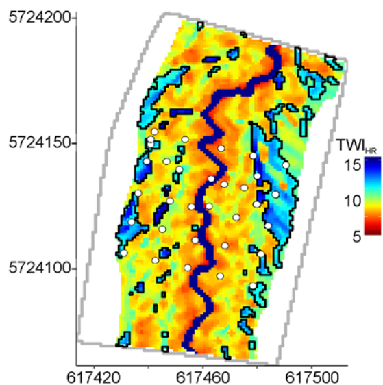
485 Figure 5. High resolution TWI ( TWI_{HR} ) map of the modeled site (excluding hillslopes). White points indicate sampling locations, the Rappbode stream is indicated by the blue line. Black polygons are high TWI_{HR} zones, indicating DOC_I source areas.
