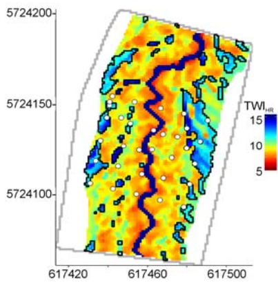
460 Figure 5. High resolution TWI ( TWI_{HR} ) map of the modeled site (excluding hillslopes). White points indicate sampling locations, the Rappbode stream is indicated by the blue line. Black polygons are high TWI_{HR} zones, indicating DOC_1 source areas.
