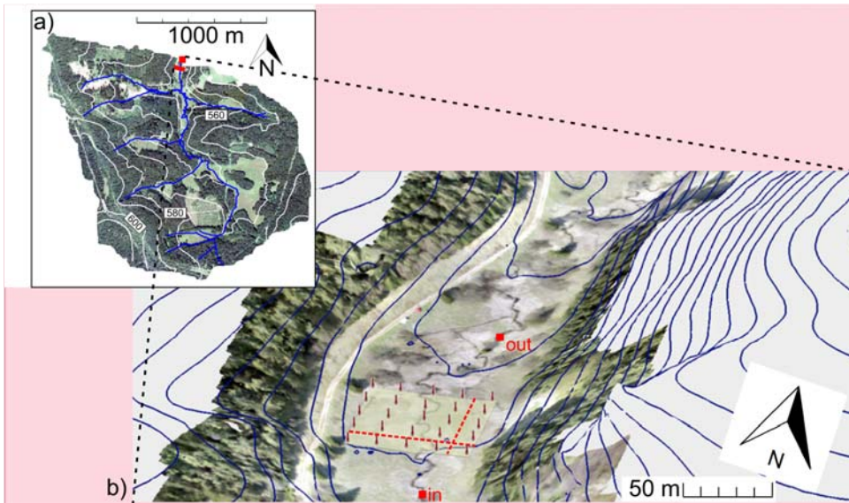
Figure 1. a) Rappbode catchment and position of the study site (red square). b) 3D view of the study site (red squares indicate in and outlet stream gauges). Red pins indicate the soil sampling transect and the piezometer network. Location of electric resistivity tomography indicated by red dashed lines. Note the 2.5-fold vertical exaggeration. Map data: ©Google, GeoBasis-DE-BKG.
