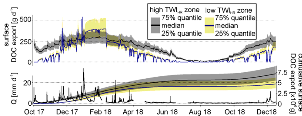
Figure 7. Absolute DOC surface export (25, 50 and 75 percentiles) from high ( \text{DOC}_I quality) and low ( \text{DOC}_{II} quality) \text{TWI}_{\text{HR}} source zones. Underlying DOC concentration percentiles based on all riparian groundwater samples of each source zone. Cumulative positive DOC export (25, 50 and 75 percentiles) from high and low \text{TWI}_{\text{HR}} zones shown on the second y axis. Discharge rate (Q) (lower black line) shown on lower left vertical axis.
