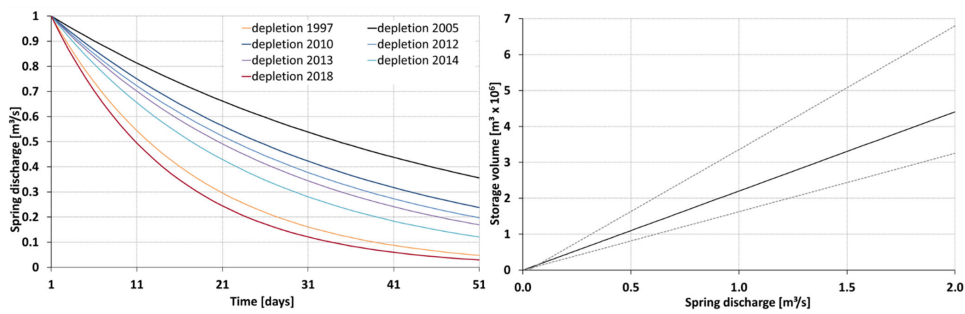
Figure 7: Depletion curves of the karst groundwater of RCZ for selected years (a) and calculated storage volumes of the groundwater body at different levels of spring discharge (b). The solid line shows the relationship for a mean recession constant "α" of 0.4 and the dashed lines are enclosing the range of one standard deviation.
