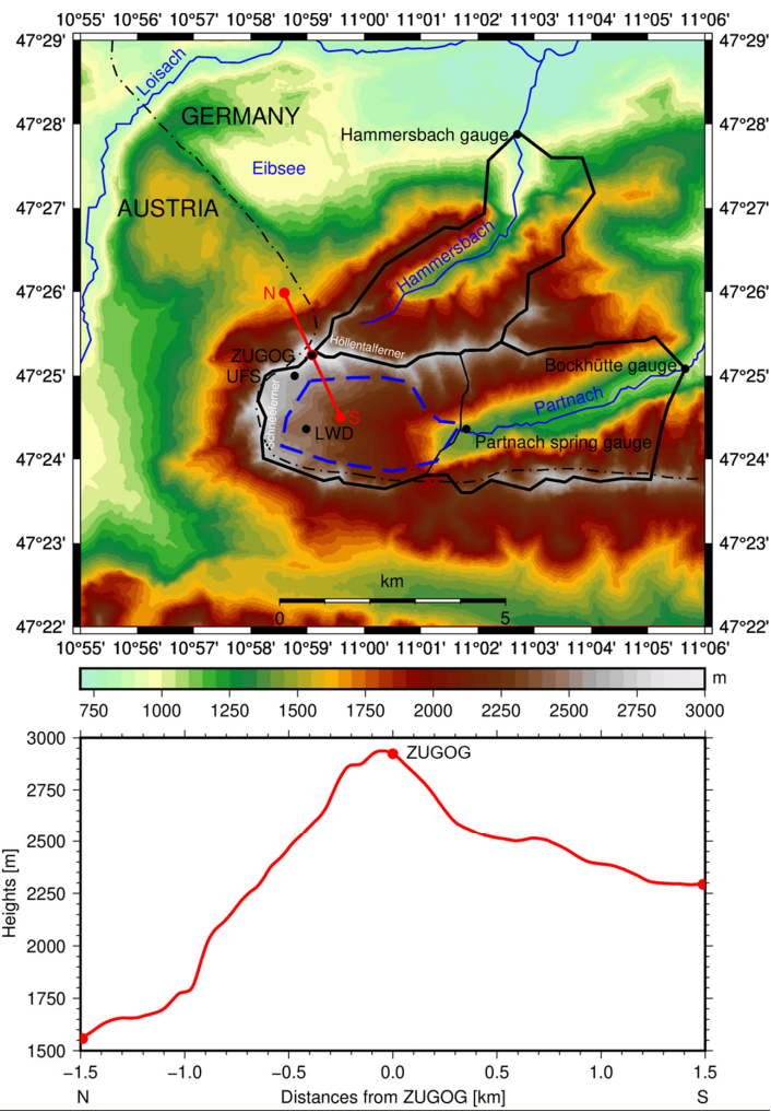
90 Figure 1: Topographic heights around the Zugspitze Geodynamic Observatory Germany (ZUGOG), the Environmental Research Station (UFS) and the hydro-meteorological station (LWD), the alpine catchments (white lines) Partnach spring (11 km 2 ) as part of Bockhütte (25 km 2 ) with their corresponding gauge stations as well as the Hammersbach catchment (14 km 2 ) with its planned gauge station, and the estimated groundwater body below Zugspitzplatt (blue dashed line) as well as a topographic profile North-South profile through ZUGOG transverse to the maximum slopes (red line)
