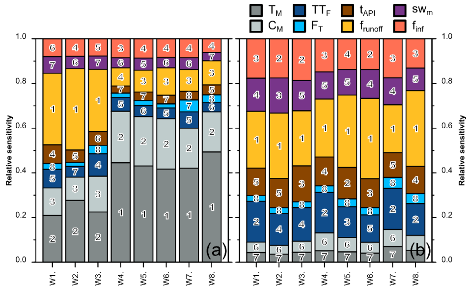
Figure 1: Relative sensitivity of the eight model parameters on the simulated river flow (a) and on the simulated potential groundwater recharge (b) for the eight groups of gauging stations. The relative parameter ranking is reported in the bars from the most sensitive, 1, to the least, 8.
