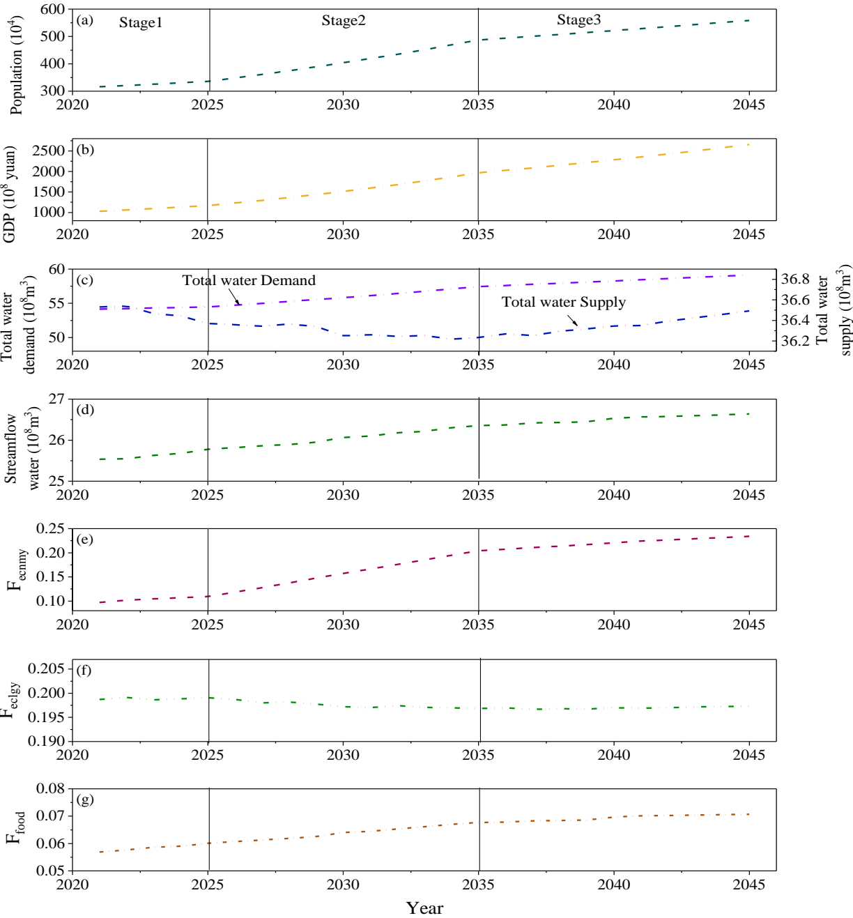
Fig.8 Coevolution process of WSEF nexus model
