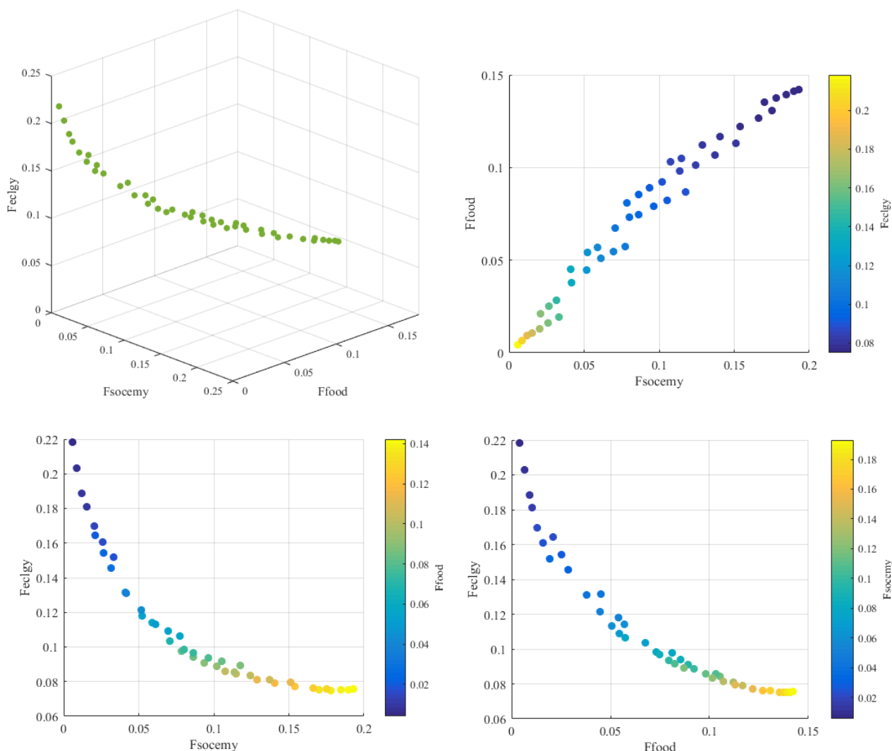
Fig.15 Portfolios of all the non-dominant optimal solutions of 2020.
