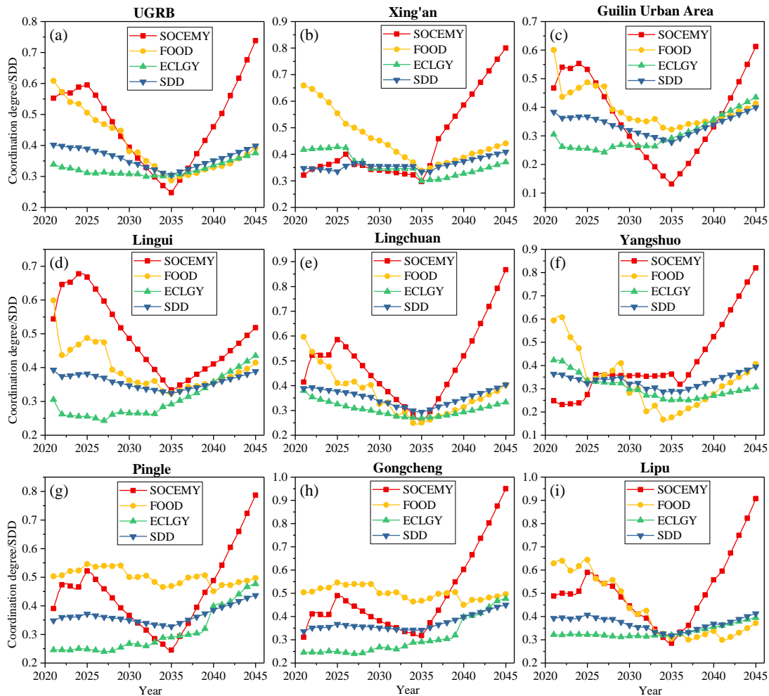
Fig.13 Time variation of sustainable development degree (SDD) of SEF nexus and coordination degree of each agent
