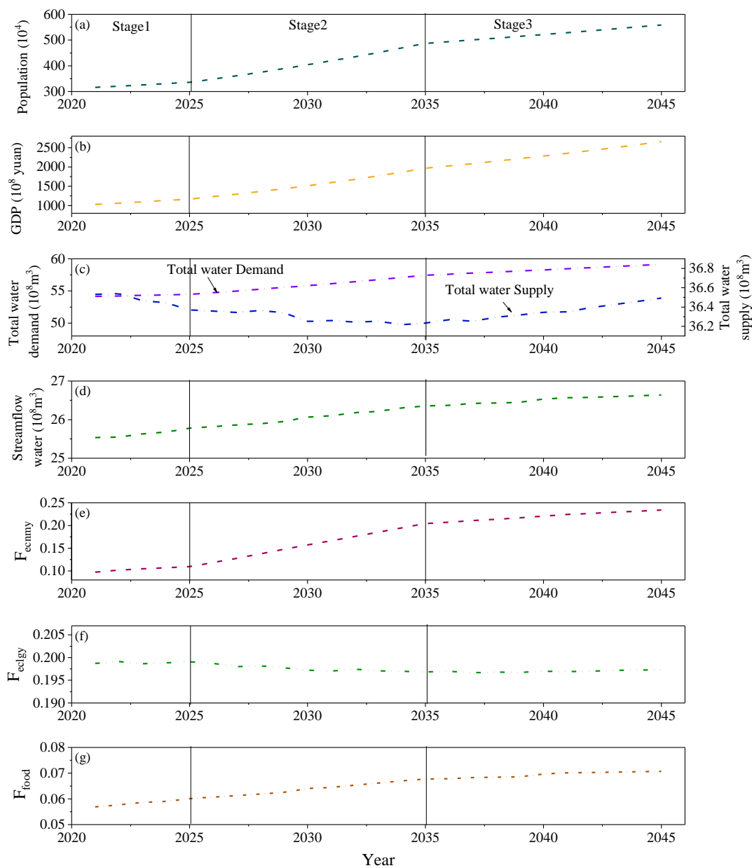
Fig.8 Coevolution process of SEF nexus model
