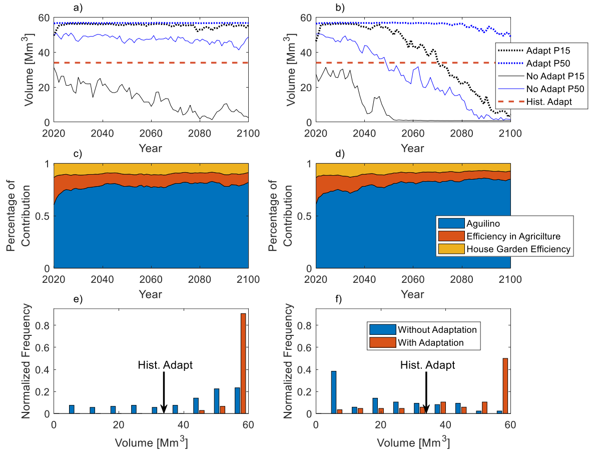
Figure 4. WEAP model water balance results under the combination of strategies; a) annual lake water volume simulated under the RCP4.5 scenario, b) same as “a)” but under RCP8.5 scenario, c) projected percentage of contribution of each strategy under the RCP 4.5 scenario, d) same as “c)” but under RCP8.5 scenario, e) normalized water volume frequency using different GCMs simulations on the period 2071-2100 under the RCP4.5 scenario, f) same as “e)” but under RCP8.5 scenario.
