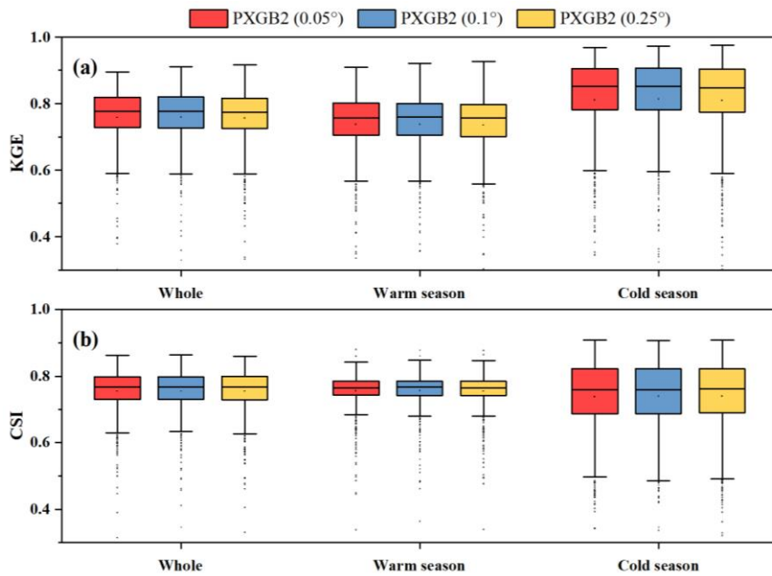
Fig. 14 The performance (KGE and CSI) of PXGB2 prepared MSPs with different spatial resolutions (0.05°, 0.1°, and 0.25°) during the whole period, warm season, and cold season.
