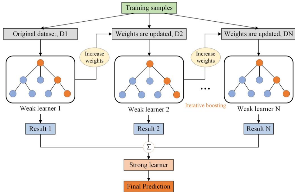
Figure4. The overview structure of GBDT.
