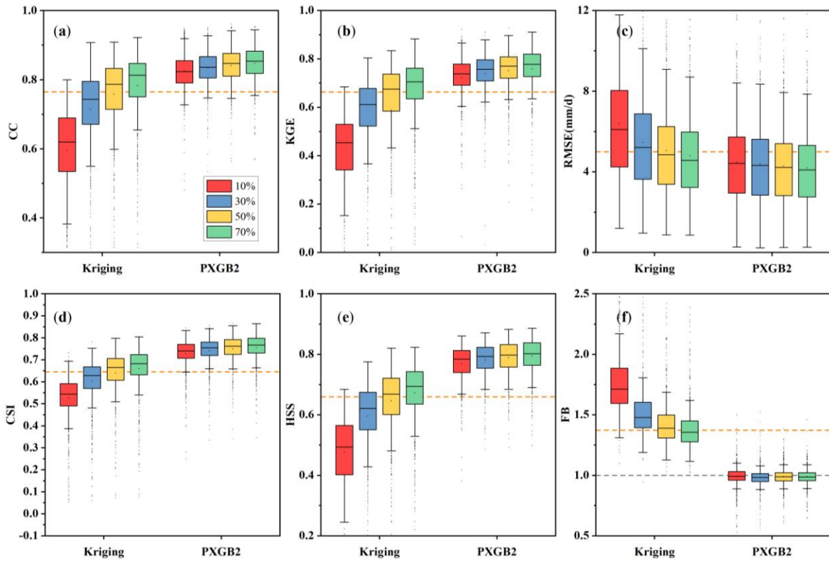
Fig. 13 Performance of PXGB2 and Kriging products using training dataset with different rain gauge densities (10%, 30%, 50, 70%). The dotted orange line shows the average of the best original product (GSMaP). The gray dotted line in (f) represents the reference line with a value of 1.
