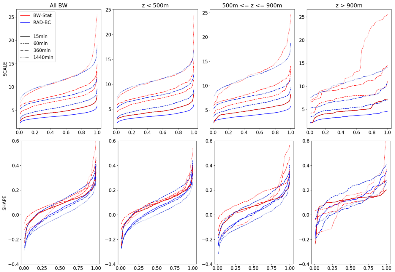
Figure 7: Spatial cumulative frequency distributions (CFD) of the scale (upper row) and shape (bottom row) parameter for the BW-Stat and RAD-BC datasets, when comparing stations and radar data at the location of all stations (left column) and for three different subsets filtered by the altitude of the respective station locations.
