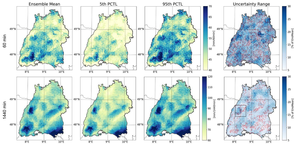
575 | Figure 6: Ensemble mean (left column) and the 5th and 95th percentiles (two middle columns) of a 100yr design storm based for two durations (60 minute events – upper row; 1440 minute events – bottom row). Additionally, the ensemble uncertainty range (difference between the 95th and the 5th percentile of the full (bootstrapping & sampling) 5000-member ensemble ) is depicted (right column). Regions with a large (> 65% of the range) contribution of the sampling uncertainty are marked with red. The black dashed square in the panel in the lower right defines the northern Black Forest region discussed in the text.
