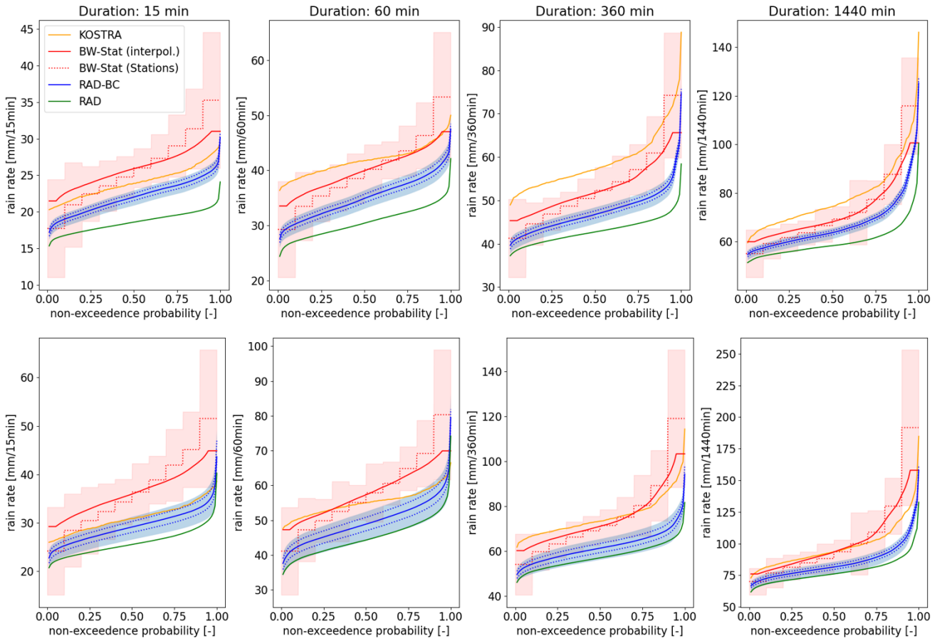
565 Figure 5: Spatial cumulative frequency distributions (CFD) of the magnitude of 20yr (upper row) and 100yr (bottom row) design storms for four different event durations and different datasets. The blue shaded range depicts the ensemble uncertainty (5th and 95th percentile of the range from the 1000 bootstraps for each of the 5 ensemble members). The dotted blue lines in the bottom row represent the range of the five ensemble members (sampling uncertainty, no bootstrapping) only. For comparison we added the interpolation error (RMSE) – red shaded area of the underlying stations (red dotted line) of the BW-Stat dataset. Note that for the 570 RAD, RAD-BC, BW-Stat (interpolated) and KOSTRA dataset the CFD are calculated on the gridded data (with fewer grid boxes in KOSTRA) while for the BW-Stat (Stations) data the stations have been binned in ten bins. In the latter dataset all stations are included in the CFD while in the gridded BW-Stat no values above/below the 5 th /95 th percentile are available.
