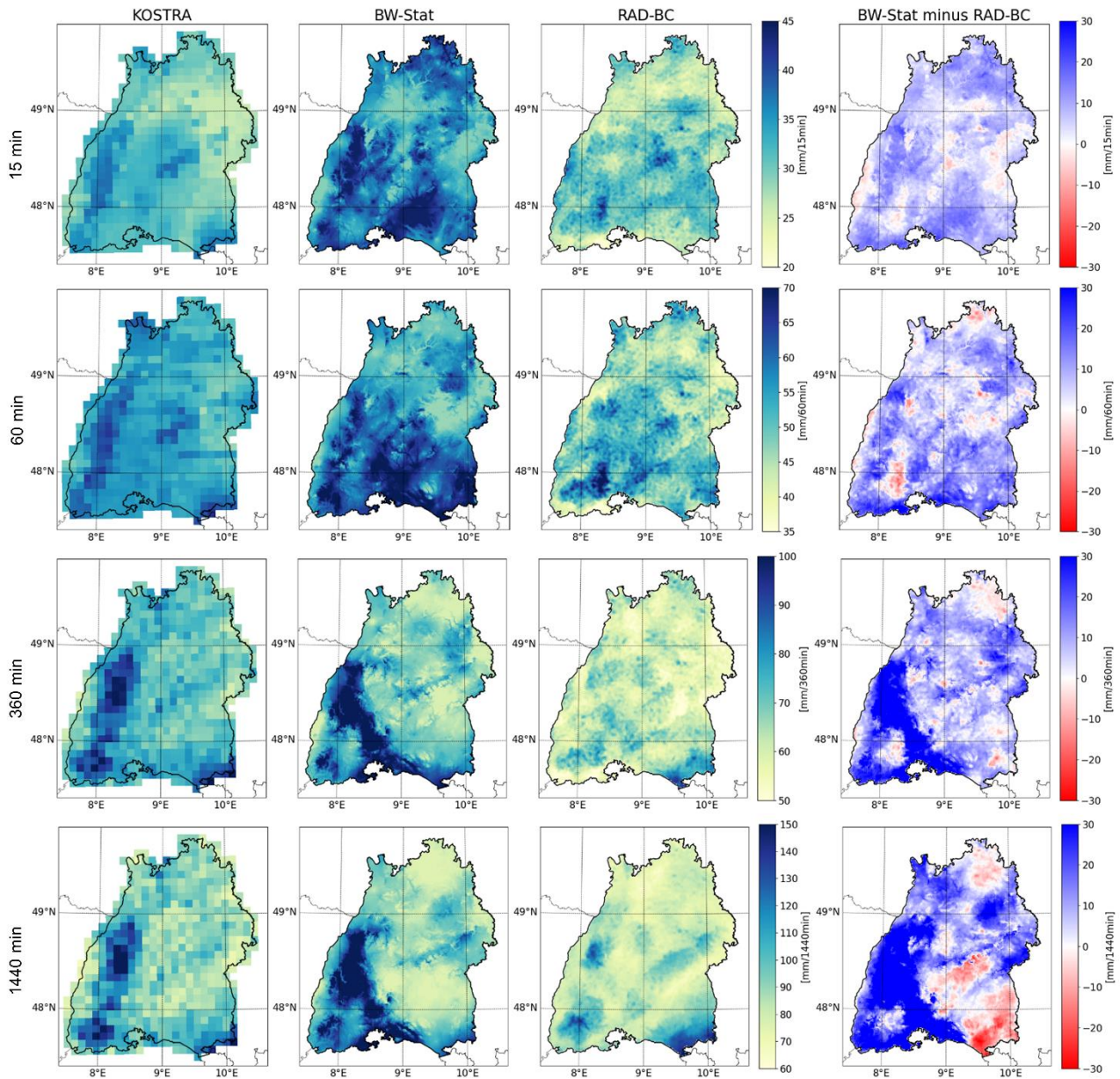
560 Figure 4: Magnitude of design storms with a return rate of 100 years for four different event durations (15, 60, 360 and 1440 minutes, depicted in rows) and three different datasets (KOSTRA, BW-Stat, RAD-BC, depicted in columns). Additionally, the difference between BW-Stat and RAD-BC is depicted (right column).
