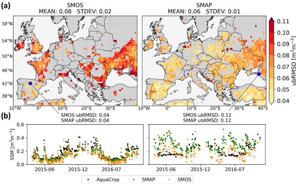
Figure 1 (a) ubRMSD of SIM1 AquaCrop SSM compared to SMOS (left) and SMAP (right) retrievals for April 2015 through December 2016. The spatial mean and standard deviation are indicated in the titles (MEAN, STDEV). (b) SSM time series of two pixels (marked by blue dots in (a) with the title indicating the ubRMSD [m 3 m -3 ] against SMOS and SMAP for each location.
