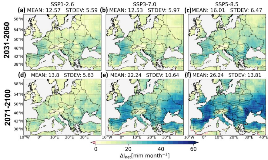
Figure 5 Changes in summer I_{\text{net}} ( \Delta I_{\text{net}} ) [mm month -1 ], median across five GCMs for the two future time horizons (rows) and the three scenarios (columns) with reference to the baseline period. The stippled areas represent pixels where all five GCMs present statistically significant changes (t-test, p < 0.05 ).
