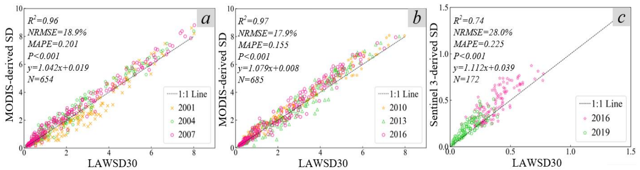
Figure 14: (a,b) Scatterplots of our LAWS30 data and the corresponding MODIS-derived SD data (Wang et al., 2020) in the 2000s (2001, 2004, and 2007) and 2010s (in 2010, 2013, and 2016), respectively; (c) scatterplot of our LAWS30 data and the corresponding Sentinel 3-derived SD data (Shen et al., 2020) in 2016 and 2019.
