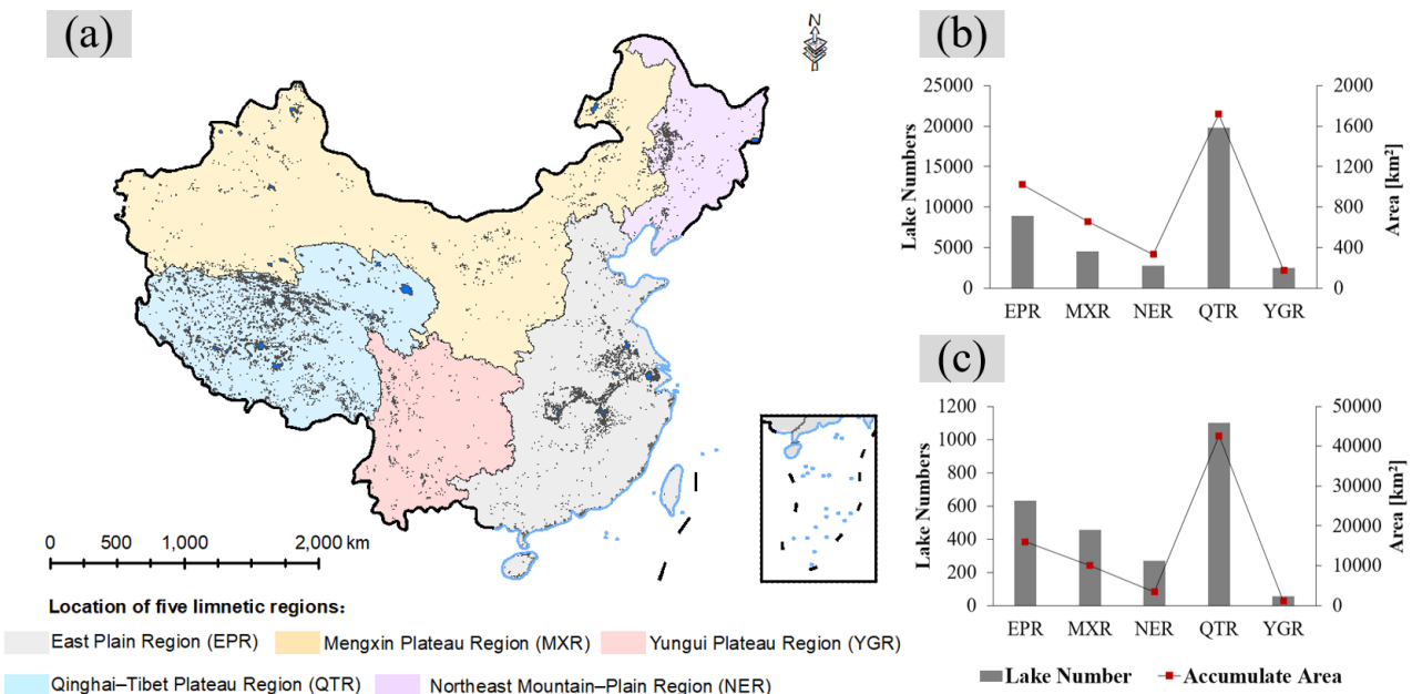
335 Figure 9: The location of the five limnetic regions and the lake statistics in each limnetic region. (a) The location of the five limnetic regions; (b) statistics of lakes with areas \leq 1 \text{ km}^2 in each region; (c) statistics of lakes with areas > 1 \text{ km}^2 in each region. The location of the five limnetic regions comes from (Ma et al., 2011; Chen et al., 2021).
