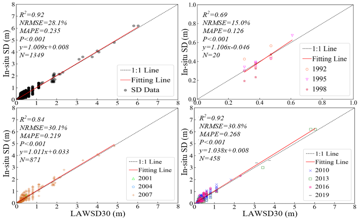
255 Figure 4: Scatterplots of the in situ measured SD data and our LAWSD30 dataset. (a) An overall scatterplot of our LAWSD30 dataset and all the collected in-situ SD data; (b–d) scatterplots of our LAWSD30 dataset and the corresponding in situ SD data in the 1990s (1992, 1995, and 1998), 2000s (2001, 2004, and 2007), and 2010s (2010, 2013, 2016 and 2019), respectively.
