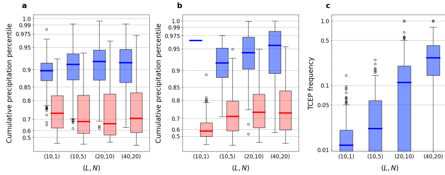
Figure A5. (a) Average percentile of cumulative precipitation during day 0-2 before and (b) during persistent high discharge periods, and (c) fraction of high discharge periods with two or more extreme precipitation events (TCEP) between day 2 before to the end of the period, averaged by catchment for the European data. In (a-b), blue (resp. red) shading indicates values that are (resp. are not) statistically significant at a 10% confidence level (see methods).
