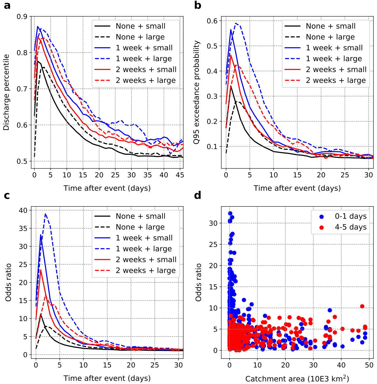
Figure 13. Daily average (a) discharge percentile, (b) probability of high discharge and (c) odds ratio of high discharge, averaged across "small" ( \text{area} \leq 10,000 \text{ km}^2 , solid lines) and "large" ( \text{area} \geq 10,000 \text{ km}^2 , dashed lines) catchments in the European data, for non-clustered (black), 1-week (blue) and 2-week (red) clustered events. (d) Average high discharge odds ratio from day 0-1 (blue) and day 4-5 (red) following an extreme precipitation event against catchment area.
